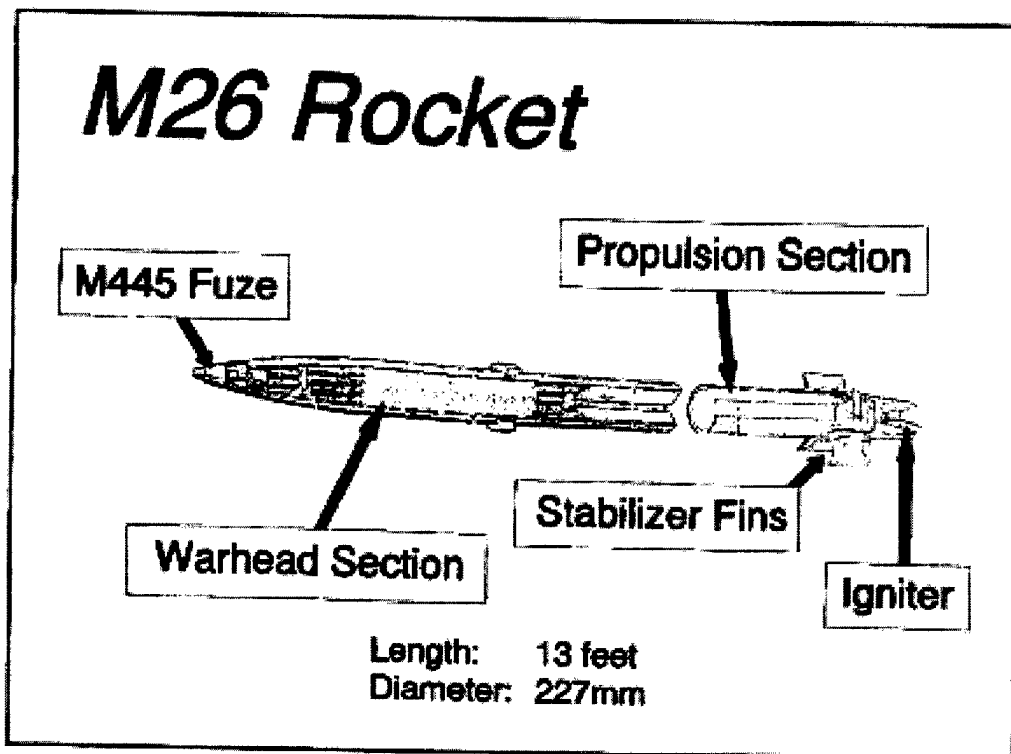
Figure 1-4. M26 rocket.
