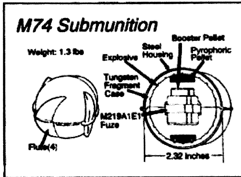
Figure 1-7. M74 submunition.
