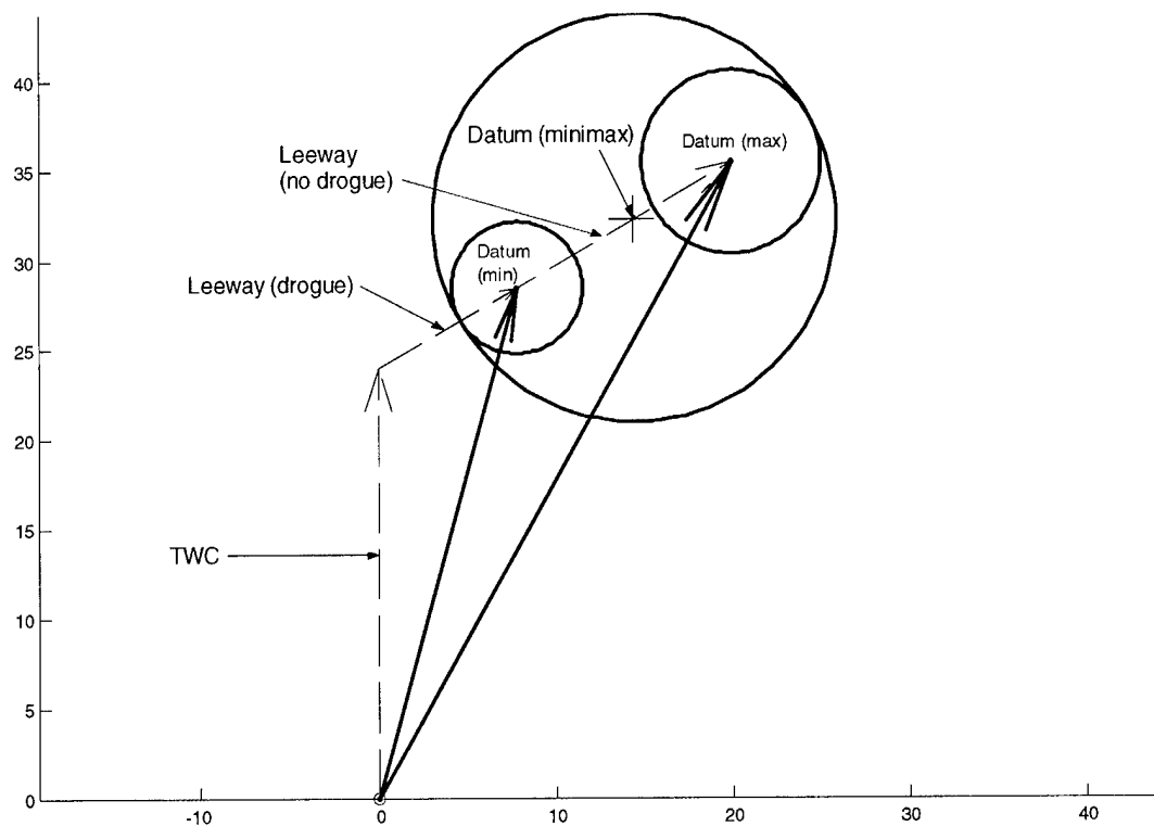
Figure 5-1. Min/Max Applied to Leeway Rate. (D_p = 0.125 \times \text{distance drifted})
