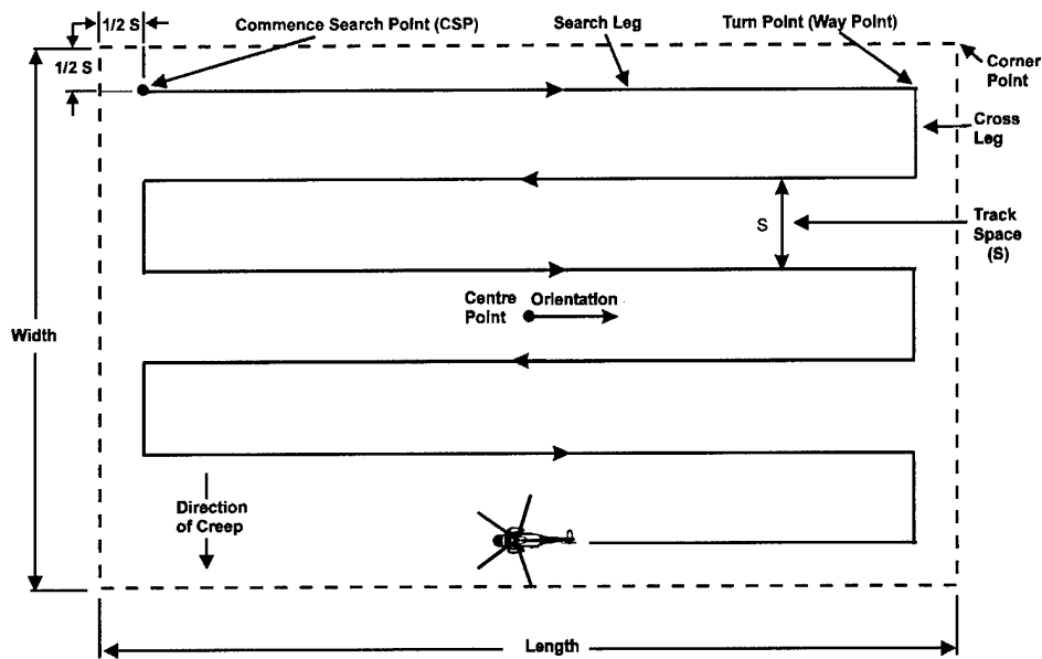
Figure 4-6. Parallel Sweep Search.
