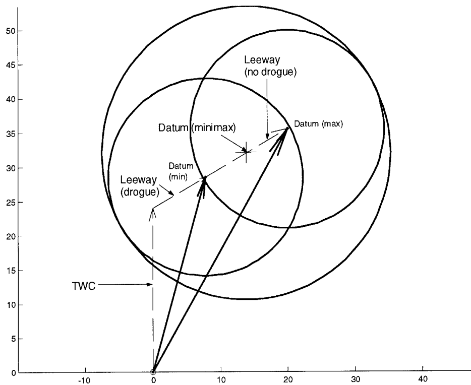
Figure 5-3. Min/Max Applied to Leeway Rate. (DV_e = 0.6 \text{ knots})
