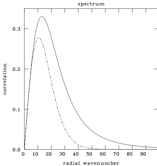
Figure F1 Radial spectrum for geostrophically-coupled SOAR model
