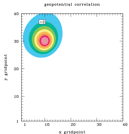
Figure 4.7 \langle \Phi \Phi \rangle correlation for variable horizontal scale
