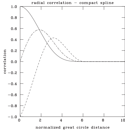
Figure A2 Compact spline function
