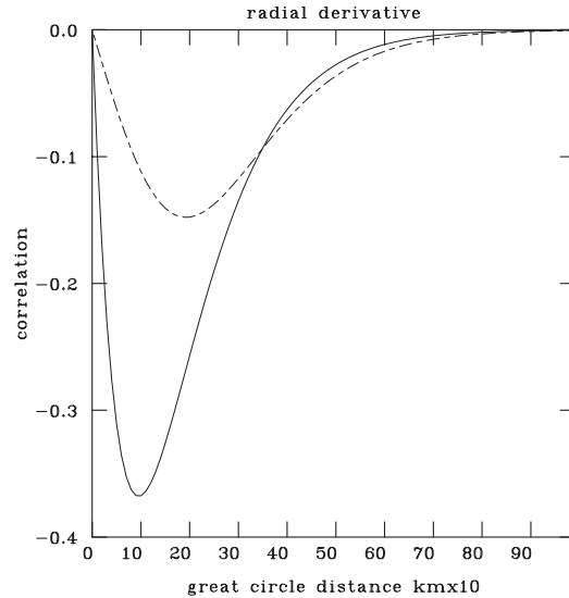
Figure F2 Correlations corresponding to the spectra of Figure F1
