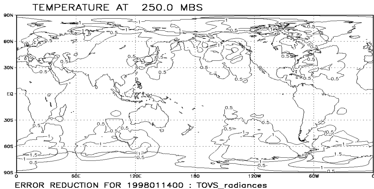
Figure 10.5b Error reduction due to TOVS radiances
