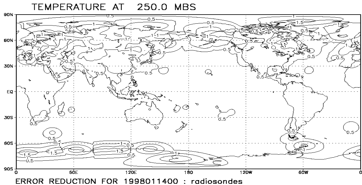
Figure 10.5a Error reduction due to radiosondes
