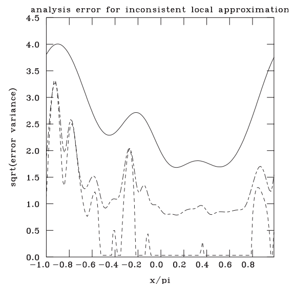
Figure 10.4 Effect of inconsistency in local approximation
