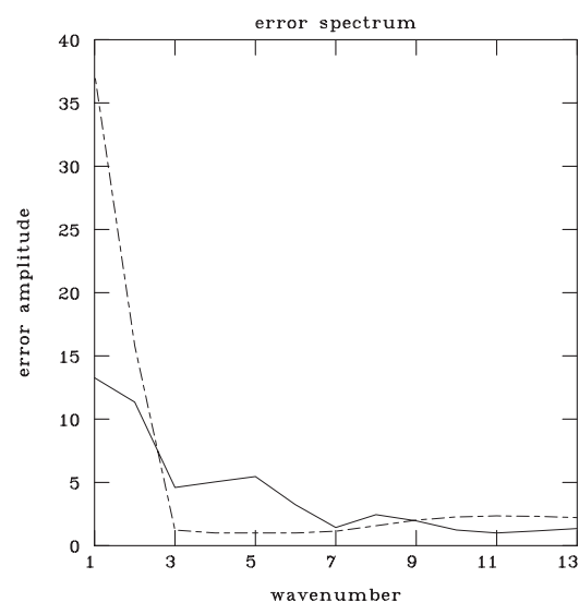
Figure 3.5 Analysis error spectra for steepest descent and standard conjugate gradient
