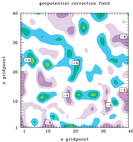
Figure 4.8a \Phi correlation for invariant horizontal scale
