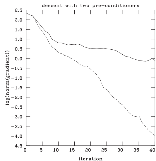
Figure 3.12 The effect of dual Choleskis
