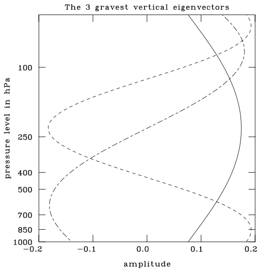
Figure 4.1 The three gravest vertical eigenvectors of \mathbf{C}_{\psi\psi}
