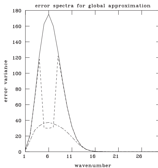
Figure 10.3b Spectra corresponding to (a)
