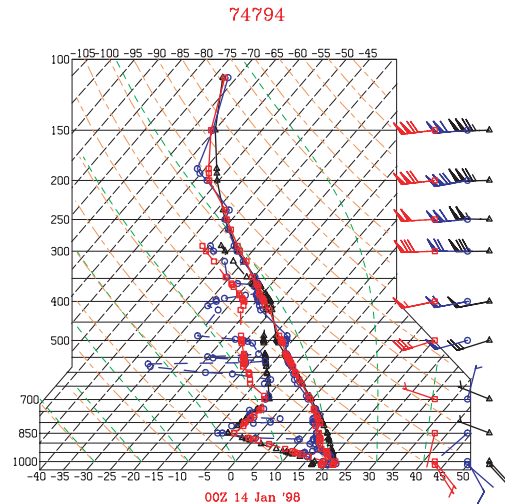
Figure 9.2 Same as Figure 9.1, except includes significant level data
