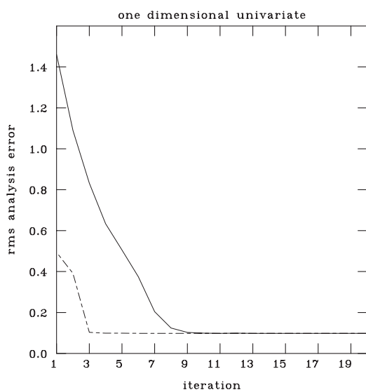
Figure 3.6 Rms analysis grid error - the effect of pre-conditioning
