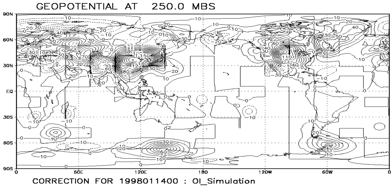
Figure 3.13b Simulated OI correction field
