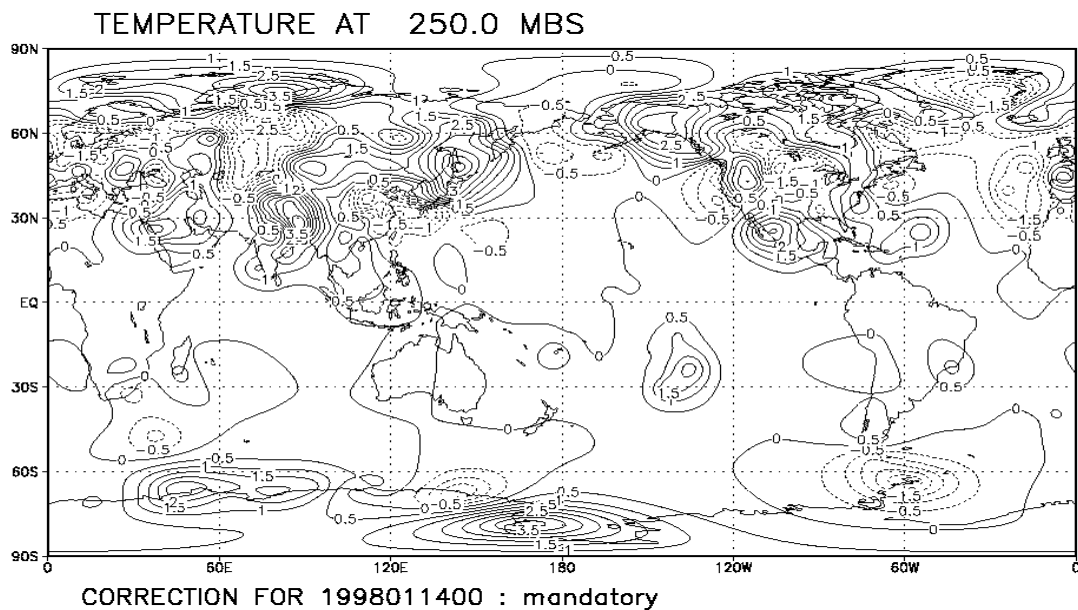
Figure 5.2b Same as 5.2a, except for mandatory only
