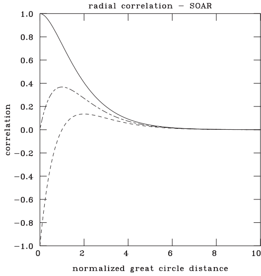
Figure A1 SOAR function
