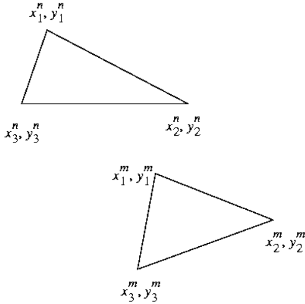
Figure E1 Labeling used for the data partition triangles (prisms)
