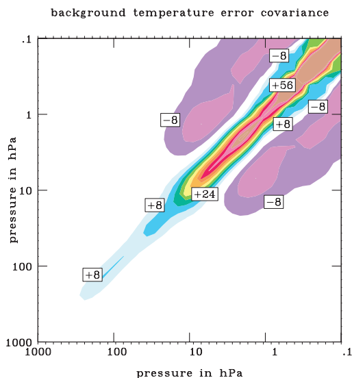
Figure 5.3 Specified <TT> background error covariance from 1000 to 0.1 mb
