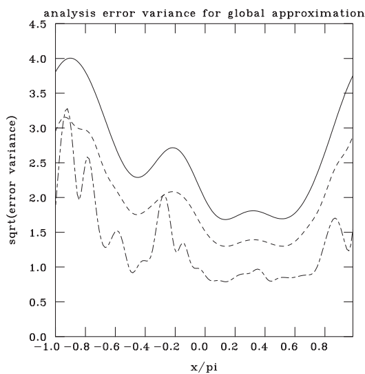
Figure 10.3a Background and analysis error variance for global approximation
