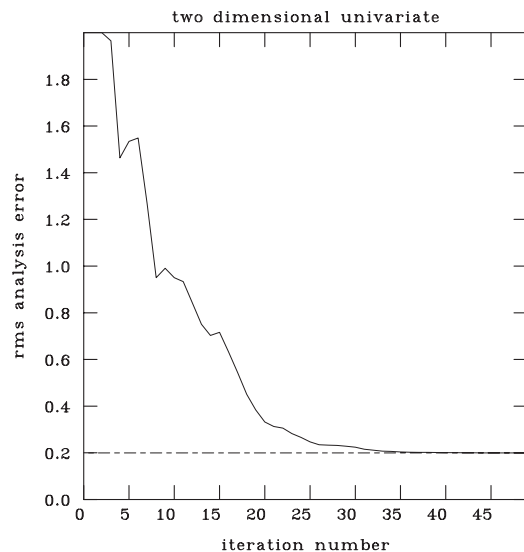
Figure 3.9 Rms analysis error (trace \mathbf{P}_a ) - conjugate gradient descent for 2D case
