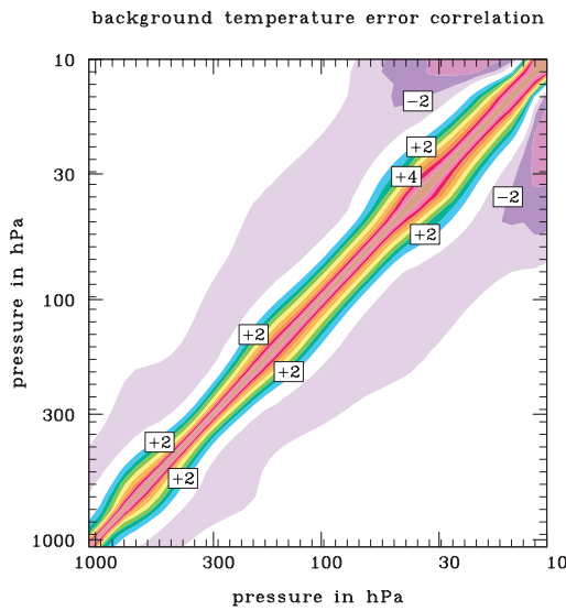
Figure 4.3 \langle TT \rangle correlation – variable vertical scale
