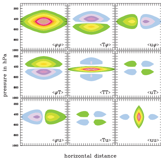
Figure 4.10a x/P cross-sections of 9 correlations – separable formulation
