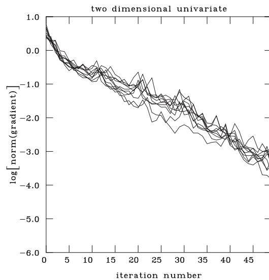
Figure 3.11 \log \|\nabla J\| for 10 realizations
