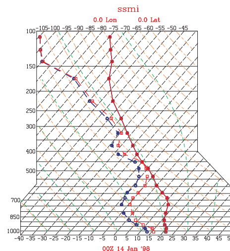
Figure 5.6 Temperature, background, and analyzed dew point from SSM/I total precipitable water
