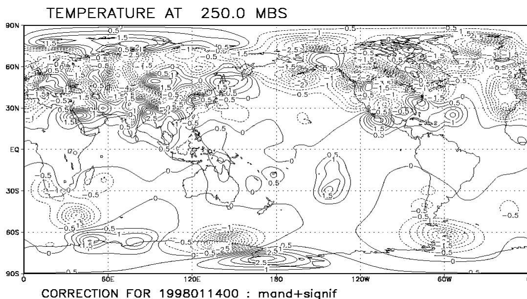
Figure 5.2a Correction fields due to radiosonde (mandatory plus significant levels)
