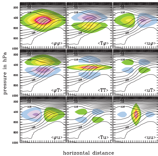
Figure 4.5 x/P cross-section of 9 correlations – pressure as vertical coordinate
