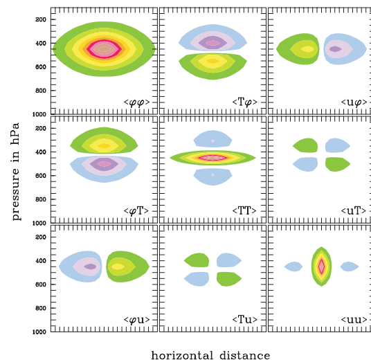
Figure 4.10b Same as Figure 4.10a, except for non-separable formulation
