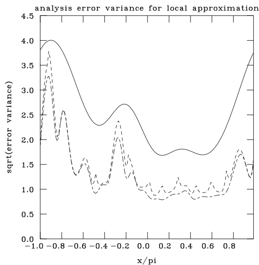
Figure 10.2a Background and analysis error variance for local approximation
