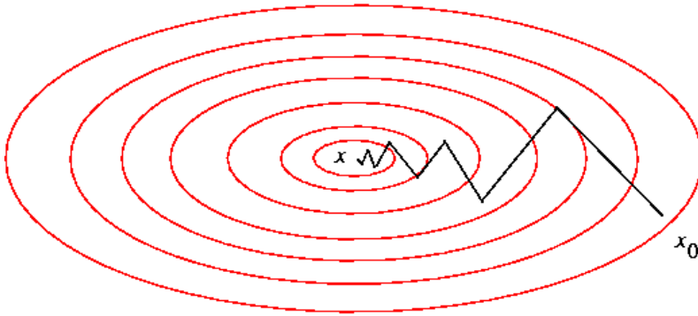
Figure 3.1 Schematic showing the iteration path for the method of steepest descent
