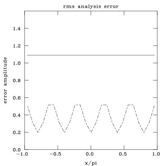
Figure 3.7 Spatial analysis error distribution at iteration 2
