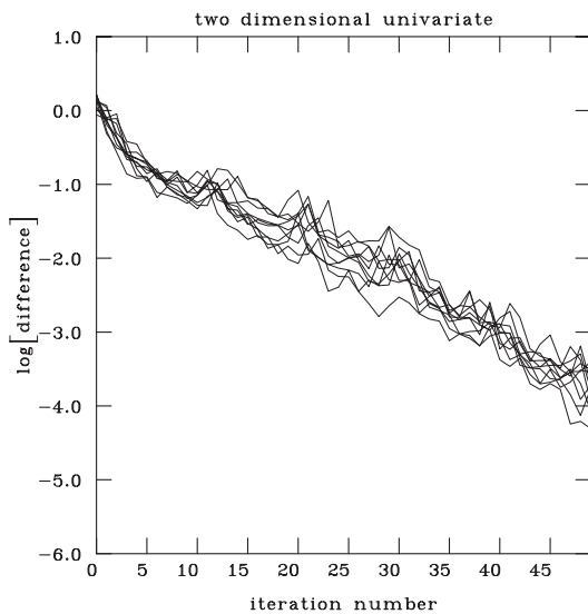
Figure 3.10 Comparison between direct solution and conjugate gradient descent
