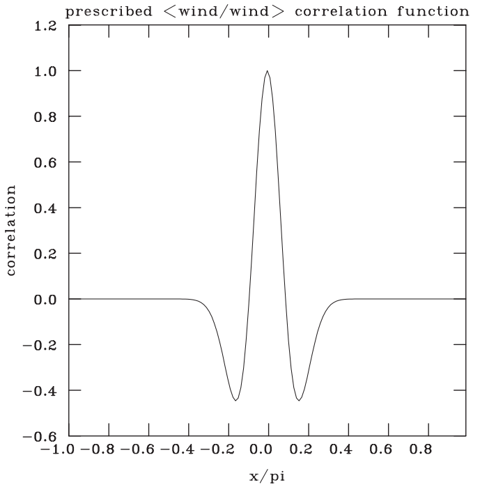
Figure 10.1 One dimensional \langle \text{wind} / \text{wind} \rangle correlation
