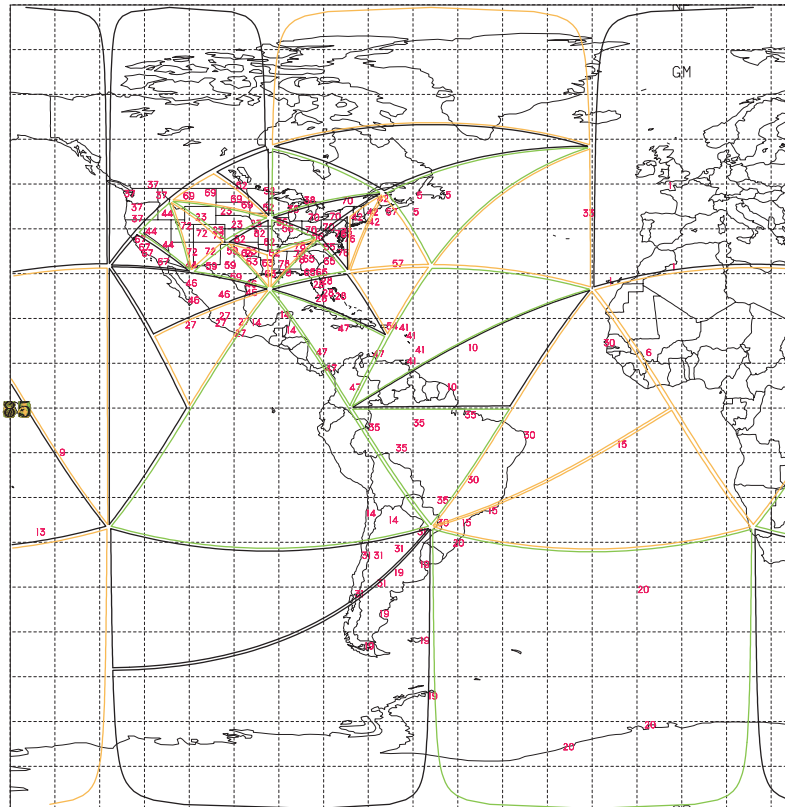
Figure 3.2 Division of the globe into triangular observation prisms
