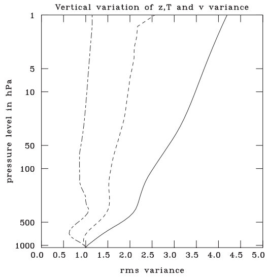
Figure 4.12 Background error variances
