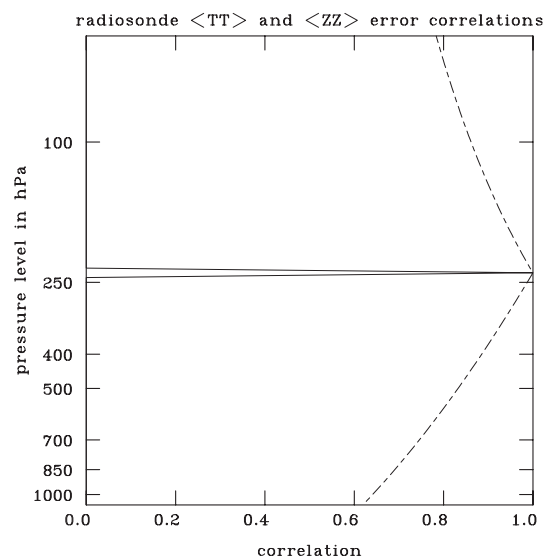
Figure 5.1 Radiosonde observation error correlations – \langle TT \rangle and \langle \Phi \Phi \rangle
