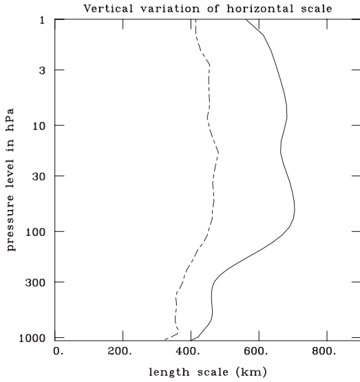
Figure 4.11 Background error horizontal correlation length
