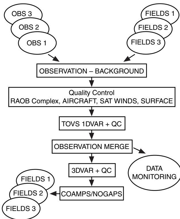
Figure 7.1 NAVDAS data flow diagram
