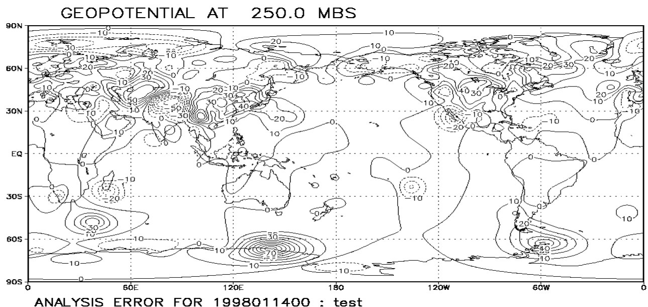
Figure 3.13a 3 DVAR correction field
