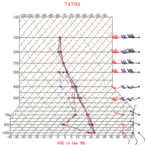
Figure 9.1 Illustration of synthetic residuals (mandatory levels only)
