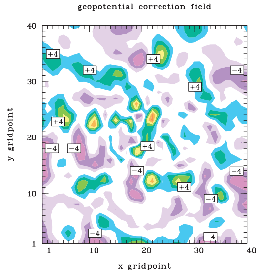
Figure 4.8b Effect of variable horizontal scale
