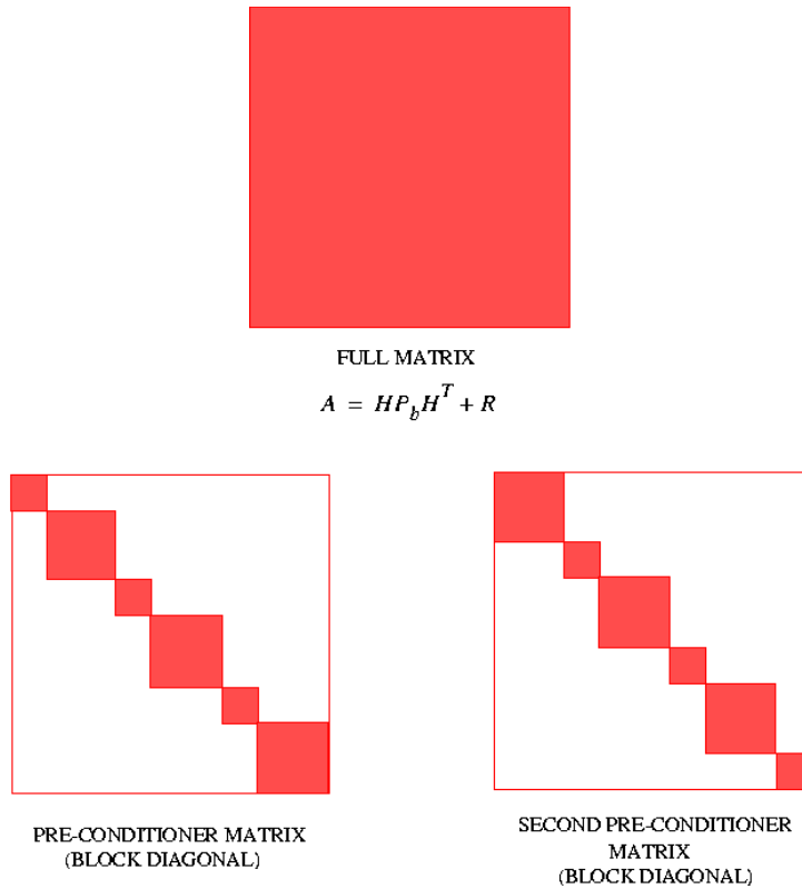
Figure 3.3 Schematic showing the full matrix \mathbf{A} and two pre-conditioners
