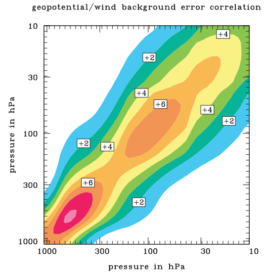
Figure 4.4 \langle \Phi v \rangle correlation – vertical geostrophic coupling
