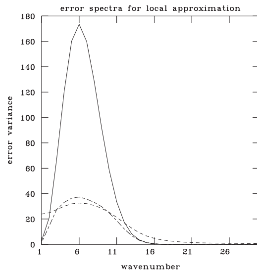
Figure 10.2b Spectra corresponding to (a)
