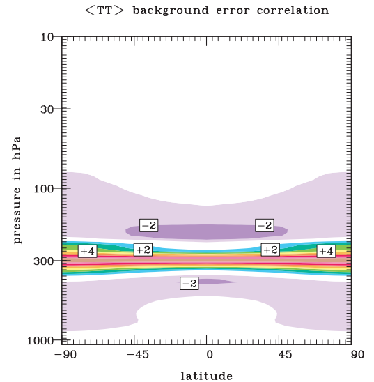
Figure 4.9 \langle TT \rangle correlation with 300 mb as a function of latitude
