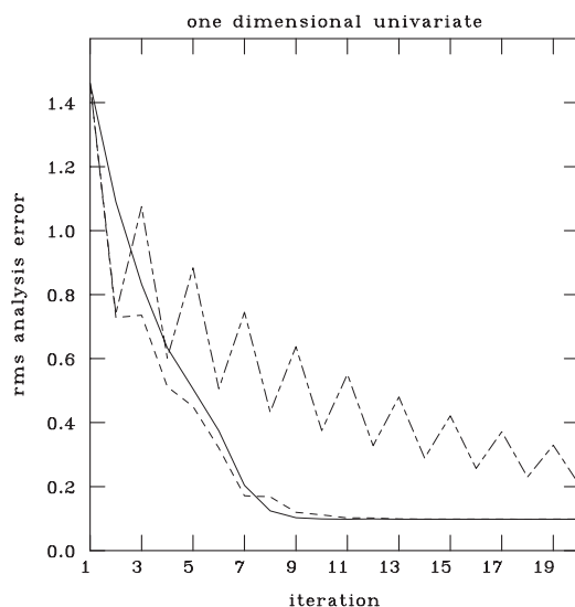
Figure 3.4 Rms analysis grid error (trace \mathbf{P}_a ) for 3 descent algorithms
