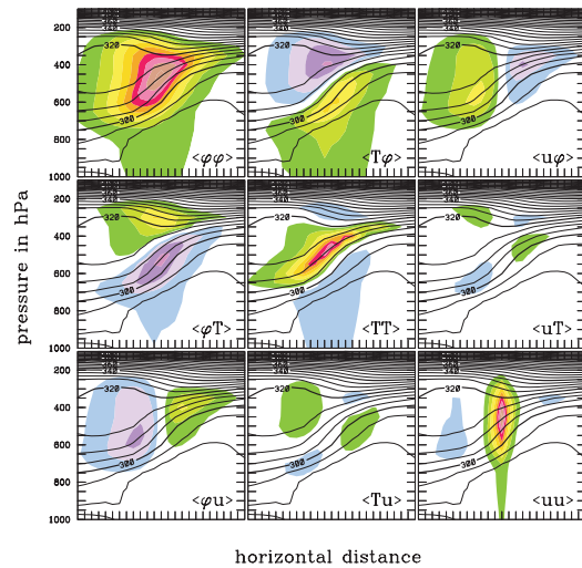
Figure 4.6 Same as Figure 4.5, except for \theta as vertical coordinate
