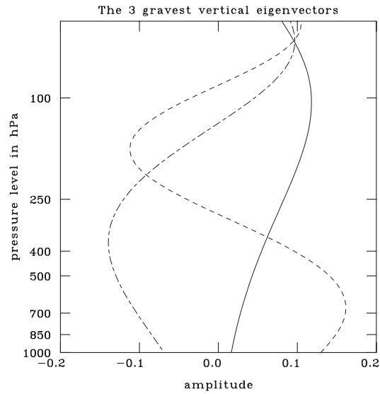
Figure 4.2 Same as (4.1) except for general \tilde{\mathbf{D}}
