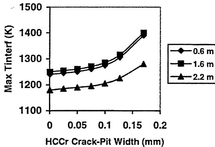
Figure 4. Typical exposed substrate interface temperature.
