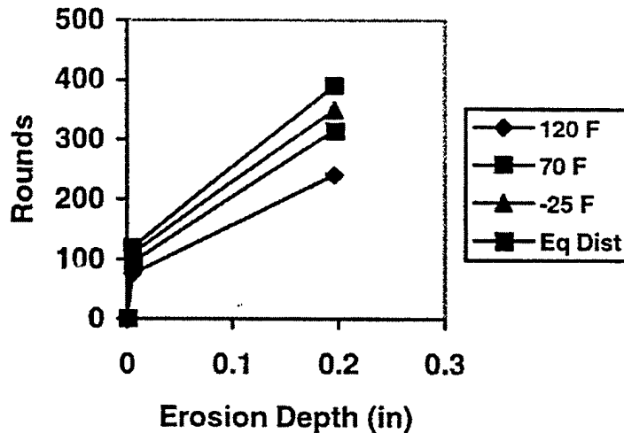
Figure 7. Ablative M256/M829E3 erosion at 60 inches from RFT.
