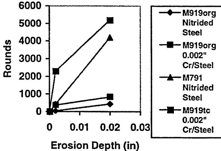
Figure 5. M242 erosion for Cycle A scenario at 6 inches from RFT.
