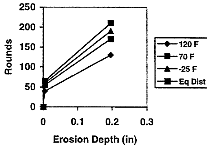
Figure 6. Nonablative M256/M829E3 erosion at 60 inches from RFT.
