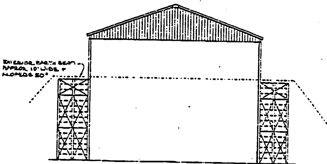
EAST ELEVATION
