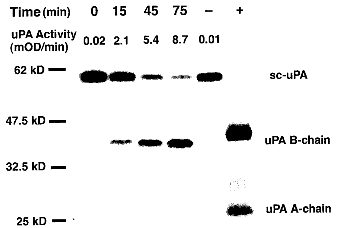
FIG. 7. Activation of sc-uPA with MT-SP1. Data from a representative experiment are shown. 5 \mu\text{M} uPA activation with 1 \text{ nM} MT-SP1 at 37^\circ\text{C} is assayed at specified times by removing aliquots and monitoring activity at 25^\circ\text{C} against the substrate Spectrozyme uK. Activity shown represents a 133-fold dilution from the original reaction mixture. Cleavage of 5 \mu\text{M} sc-uPA with 1 \text{ nM} MT-SP1 at 37^\circ\text{C} is examined over time using immunoblot analysis. sc-uPA is cleaved into an A-chain and B-chain upon activation. Native, active uPA, which is used as a control (+), has different glycosylation compared with recombinant sc-uPA used in the assay, leading to differences in molecular weight. Unreacted sc-uPA incubated under the same conditions is shown in the - lane.
