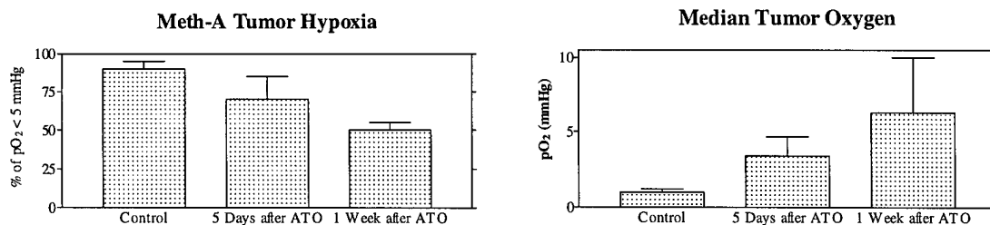
Figure 2. Oxygen polarographic measurements following ATO administration. Tumor oxygen was measured in over 100 locations in 8 to 10 tumors. The values presented represent average values and standard error of the means.
