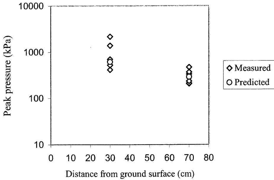
Figure 8: Peak pressure at transducers 1 and 2 positions, DOB = 3cm
