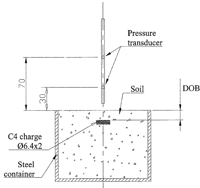
Figure 1: 100g simulated anti-personnel (AP) mine charge – configuration of experiment (unit in cm)
