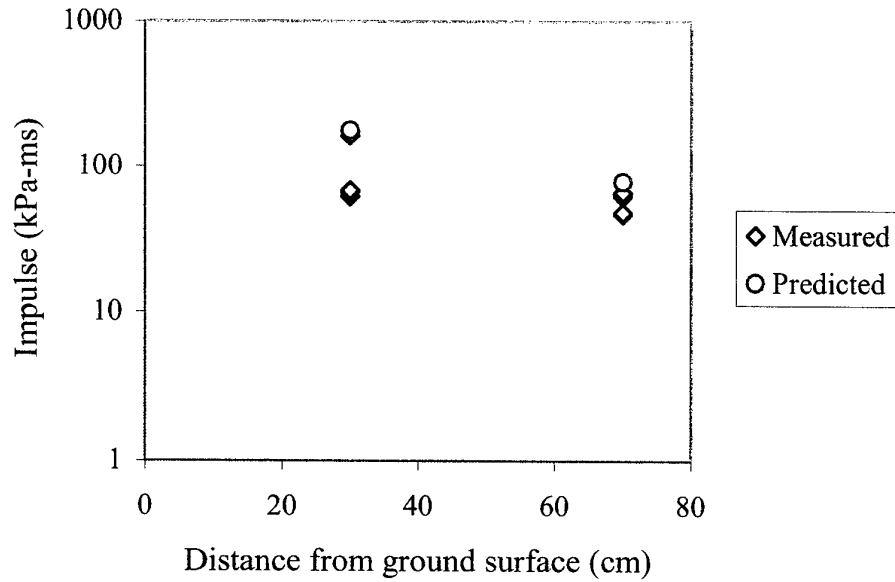
Figure 9: Impulse at transducers 1 and 2 positions, DOB = 3cm.
