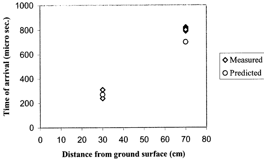
Figure 7: Time of arrival at transducers 1 and 2 positions, DOB = 3cm.
