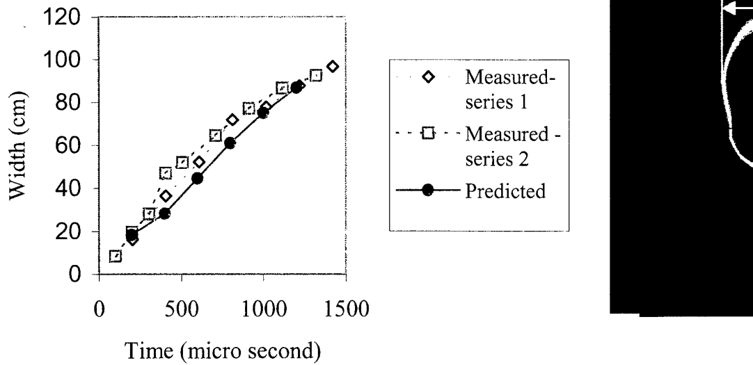
Figure 13: Width of detonation products cloud, DOB = 3cm
