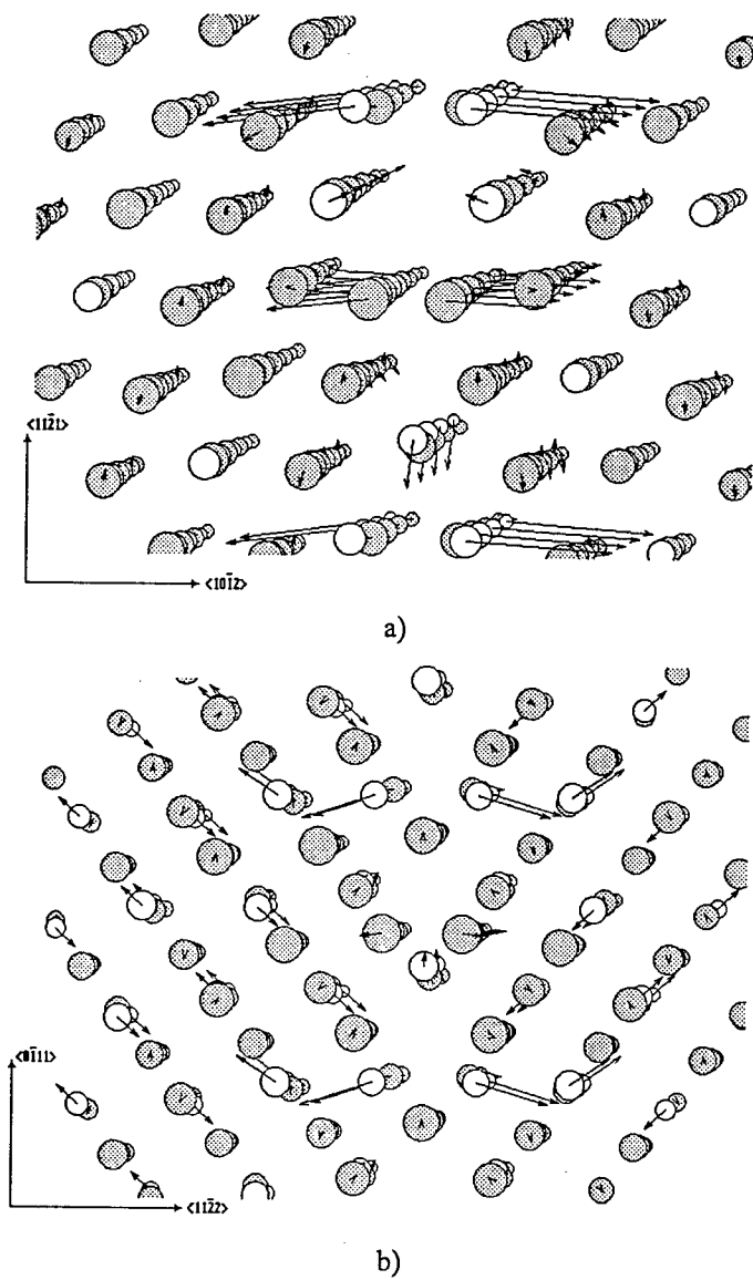
Fig. Patterns of atom configurations and microdeformations of Ti_3Al alloy lattice near the twins projection on the plane: a) (1\bar{1}00) , b) (\bar{1}100) . The scale of atomic displacements: a) 8:1, b) 4:1. White circles – atoms of Al, grey circles – atoms of Ti.
