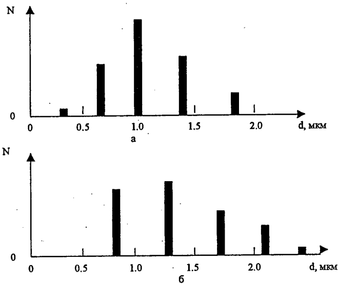
Figure 1. Histograms of a grain size of the submicro-grained aluminium rod (a diameter -7 mm): a- cross-ways the axle of a rod; б- along the axle of a rod.
