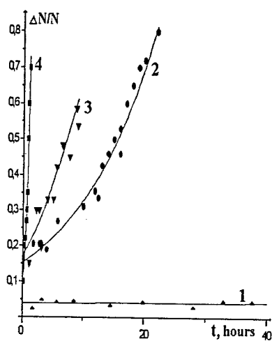
Fig. 2. The relationship between comparative changing of dislocations number at crack tip ( \Delta N/N ) and time ( t ) of treatment: 1. T=355 K, 2. \lambda=760 nm, 3. \lambda=350 nm, 4. \lambda=0,154 nm.
