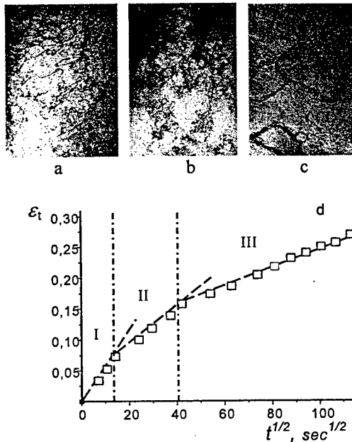
Fig.1. The dislocation structure evolution o copper during low-frequency shock treatmen (0,8 Hz) ( \times 19000 ): a) \varepsilon_t=0,03 ; б) \varepsilon_t=0,1 ; в) \varepsilon_t=0,25 ; г) strain hardening curve i coordinates \varepsilon_t - t^{1/2} .
