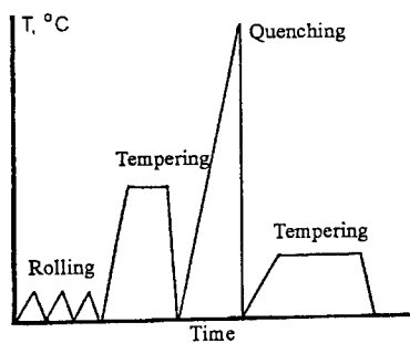
Fig.1. The technological scheme of goods production.
