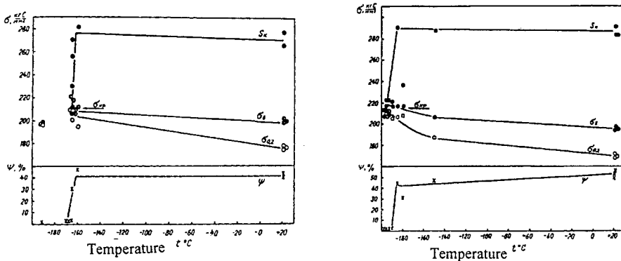
a b Fig.2. The results of mechanical testing of thermal hardened 45XH2MΦA steel without rolling (a) and with rolling (b): \epsilon_1=5...7\% , \epsilon_2=53\% .
