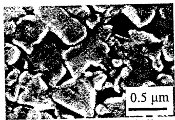
Fig 1. The structure of alloy WC-6%Co by mas., d = 0.33 \mu\text{m} .
