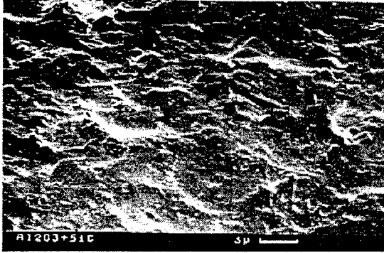
Fig.2. SEM of fracture surface of Al 2 O 3 -5wt.%SiC composite.
