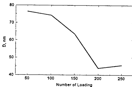
Fig. 2. Changes of size of koherent blocks during loading.
