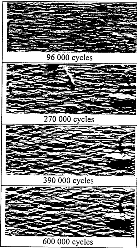
Fig. 1. Evolution of sensor surface relief ( \langle 001 \rangle \{100\} , 146 MPa, 512x200 pixels)
