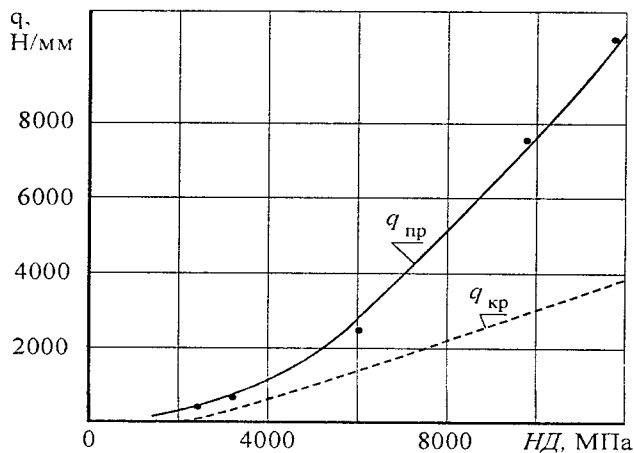
Fig. 1. Specific loading (limiting q_{np} and critical q_{кп} ) in contact of a cylindrical roller ( R=5 mm) with details of different hardness HД ; the solid line – account q_{np} agrees [3], point – experiment; the dotted line – account q_{кп} agrees [1].
