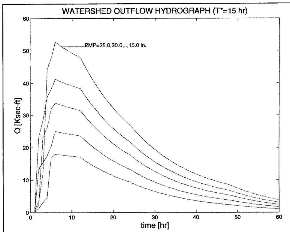
Figure 15. Family of reservoir inflow-flood hydrographs built for a deterministic watershed with a relatively long centroidal lag time ( T^* = 15 hr) for several values of the water-input event PMP
