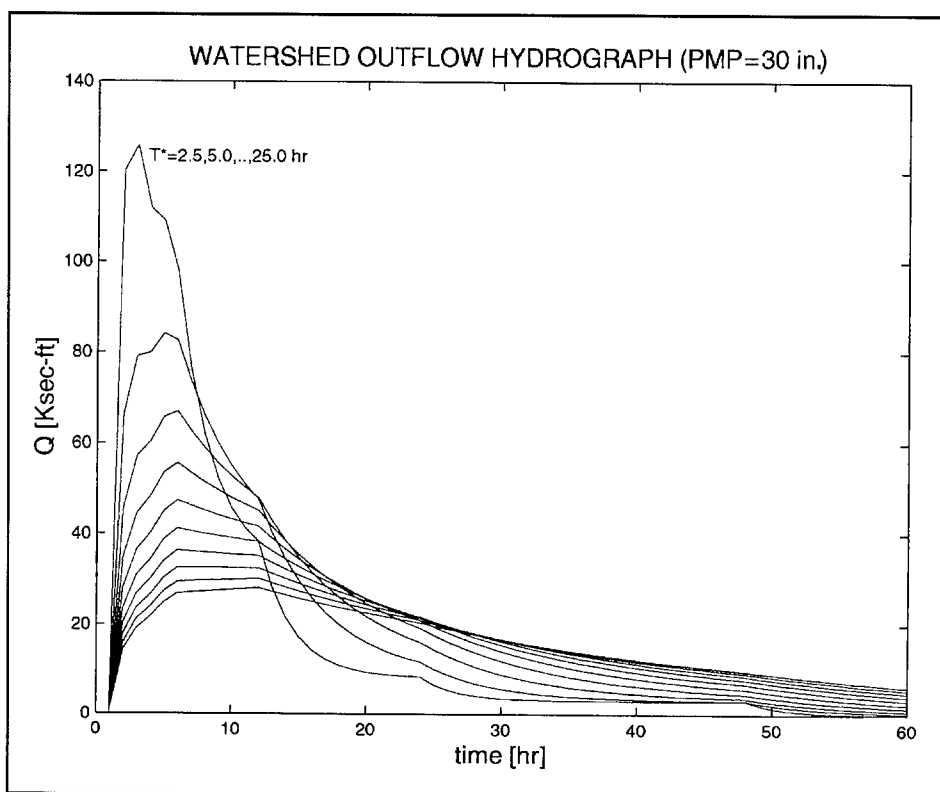
Figure 9. Family of traces of the hydrograph surface shown in Figure 7 with a set of planes T^* = \text{constant}
