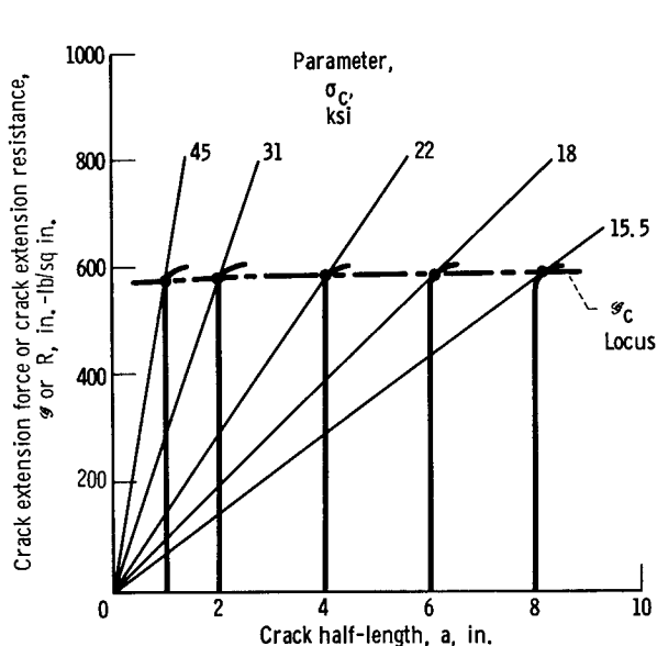
Figure 3. - Showing near-invariability of \mathcal{G}_c as function of initial crack length for material having crack extension resistance curve of near-ideal-brittle type.
