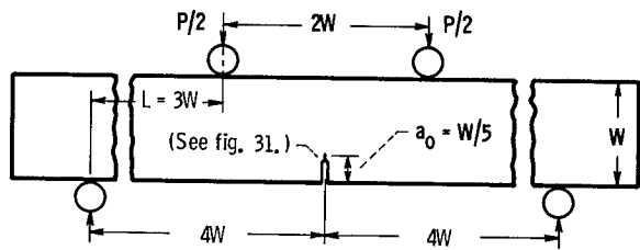
(c) Notch bend specimen (four-point loaded).
