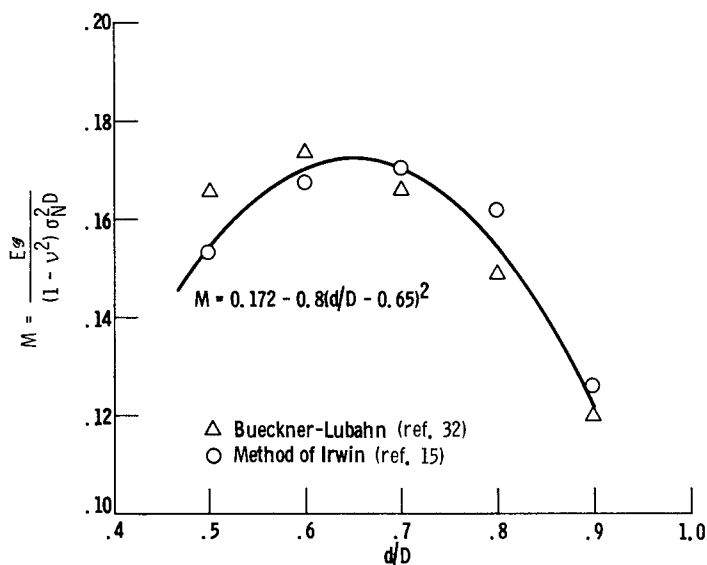
Figure 20. - Values of dimensionless factor M for round notched bars as function of d/D . Eg_I = M\sigma_N^2 D(1 - \nu^2) .
