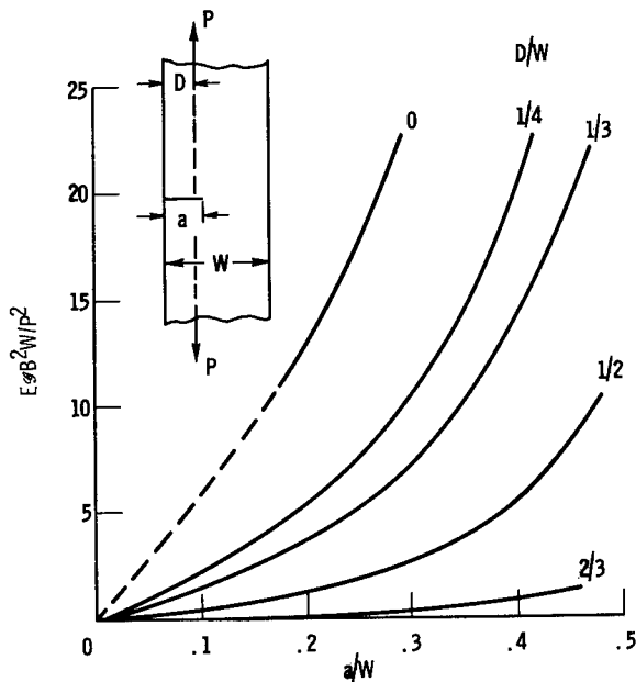
Figure 17. - Dependence of relation between dimensionless calibration factor E\epsilon B^2 W/P^2 and a/W for single-edge-notched tension specimens on location of axis of loading as specified by parameter D/W .
