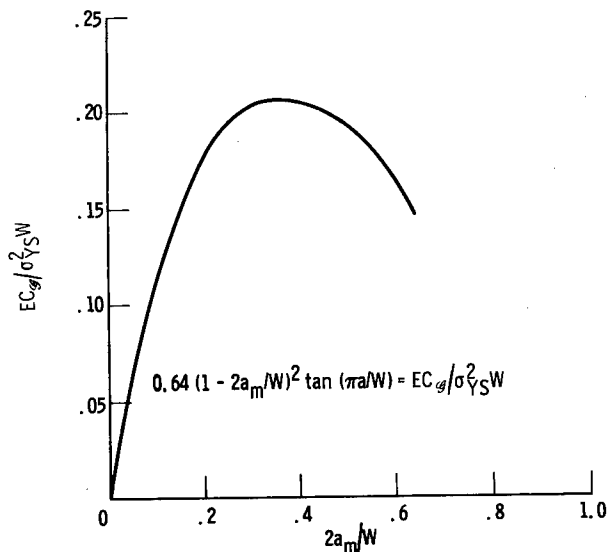
Figure 13. - Dependence of EC_g/\sigma_{YS}^2 W for symmetrically center-cracked specimens on 2a_m/W , where C_g is estimate of maximum value of \mathcal{G}_c that can be measured with acceptable accuracy for given values of W , E , and \sigma_{YS} (see text).
