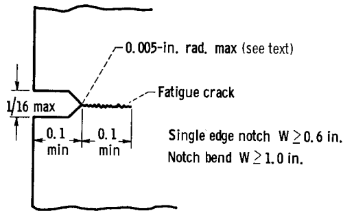
(b) Fatigue crack starter for edge-notched plate specimens.
