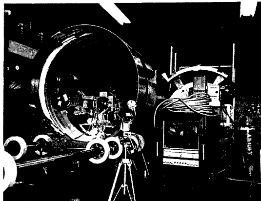
[SEAM WELDING] 2, p. 5 FIGURE 2.—Overall view of metal-inert-gas welding equipment including the seam tracker, the proximity control unit, and a closed-circuit television hookup.
