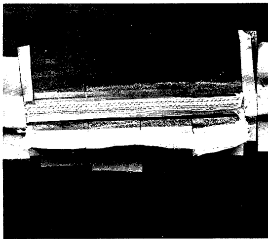
FIGURE 20.—Welded seam backed up with one type of fiber-glass tape. The texture of the tape was retained by the bead.
