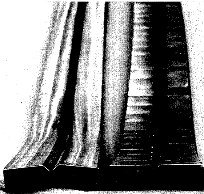
FIGURE 14. —Segmented backup bars shown side by side. Note the two-piece construction of the 0.040-inch bar on the left as compared with the unit construction of the \frac{1}{2} -inch segments on the right.
