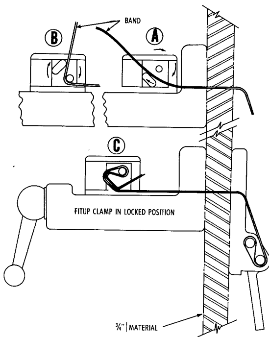
FIGURE 32.—Band installation in sequence.
