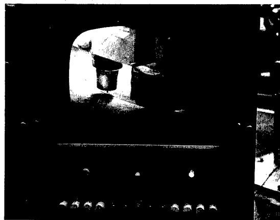
FIGURE 4.—Closed-circuit television closeup of a metal-inert-gas weld in progress using the seam tracker and the proximity transducer.
