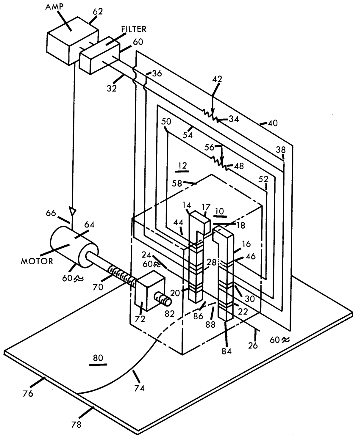
FIGURE 1.—Drawing of seam tracker.
