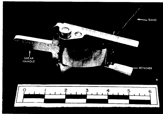
FIGURE 28.—Assembly of fitup tool.
