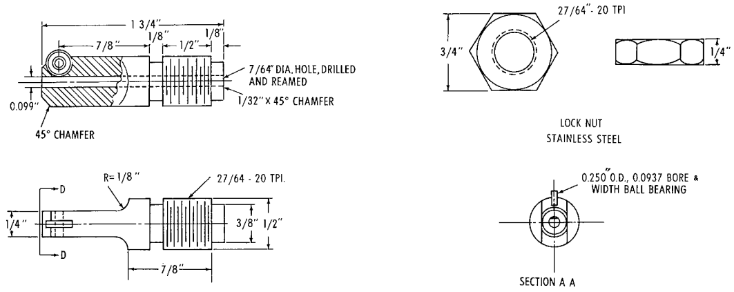
FIGURE 36.—Blueprint drawings of guide tip for feeding filler wire. Material for tip body to be copper.
