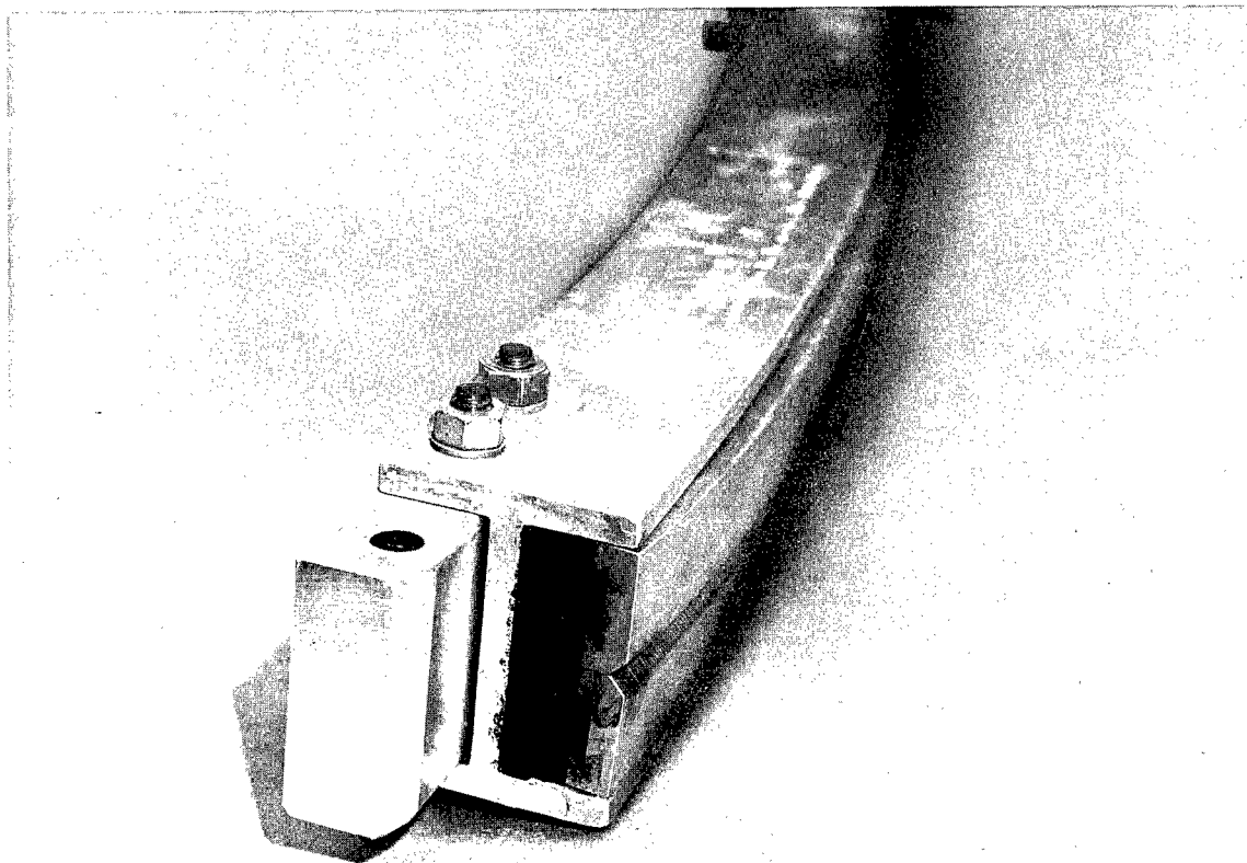
FIGURE 12.—A 41-inch segment of an "H" member showing the end of the inflatable bladder in the laminated 0.040-inch stainless-steel, backup bar bonded to silicone rubber.
