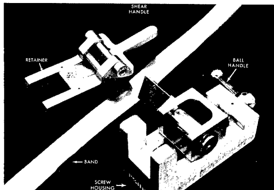
FIGURE 24.—Components of the fitup tool.
