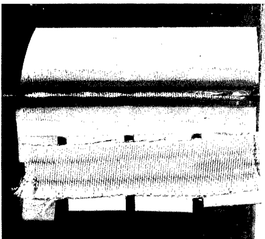
FIGURE 19.—1/4-inch 2219-T87 aluminum-alloy plate welded with fiber-glass backup tape. The tape has been pulled back to expose the inner bead.
