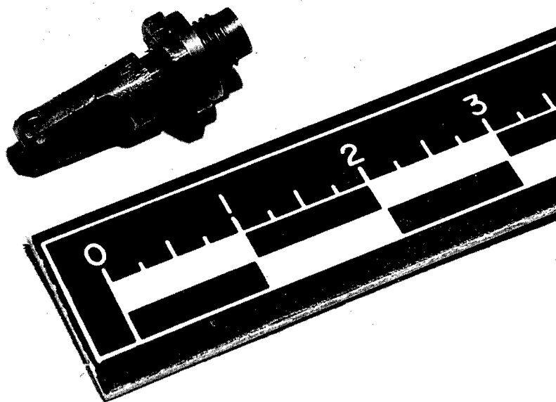
FIGURE 35.— Guide tip for feeding wire when welding with the metal-inert-gas process. Note the ball bearing in the tip.
