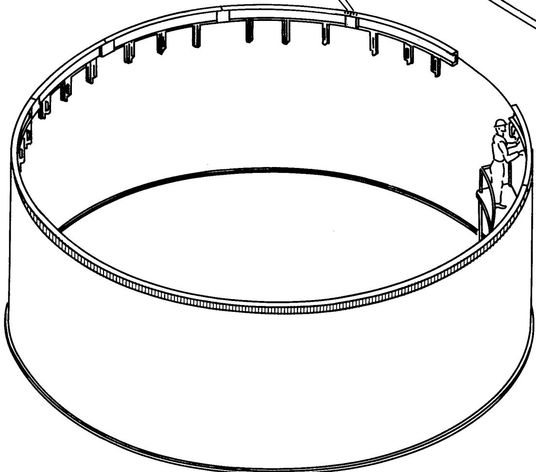
FIGURE 10.—Installing backup bar sections.
