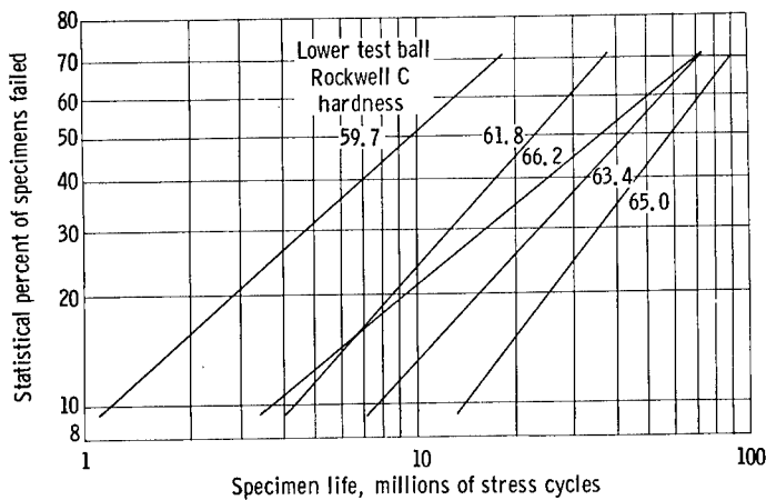
Figure 2. - Summary of rolling-contact fatigue lives of five-ball system composed of SAE 52100 steel lower test balls of varying hardness run with Rockwell C hardness 63.2 SAE 52100 steel upper test ball at a maximum Hertz stress of 800,000 psi. Room temperature; highly purified naphthenic mineral oil. (Data taken from ref. 2.)
