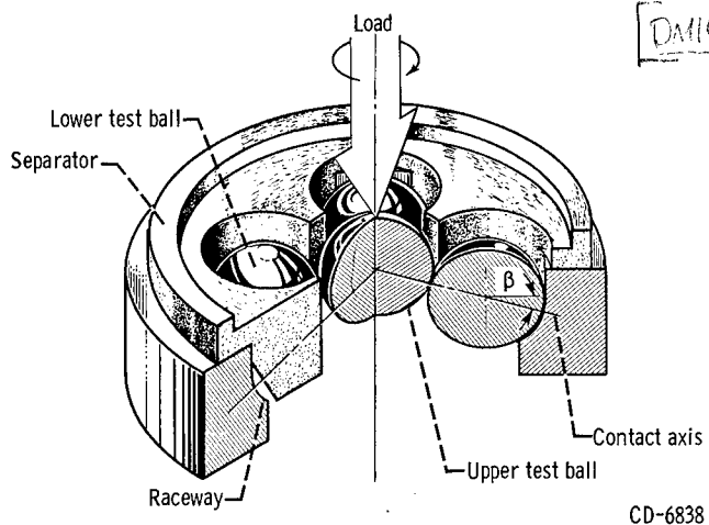
(b) Schematic of five-ball fatigue tester.
