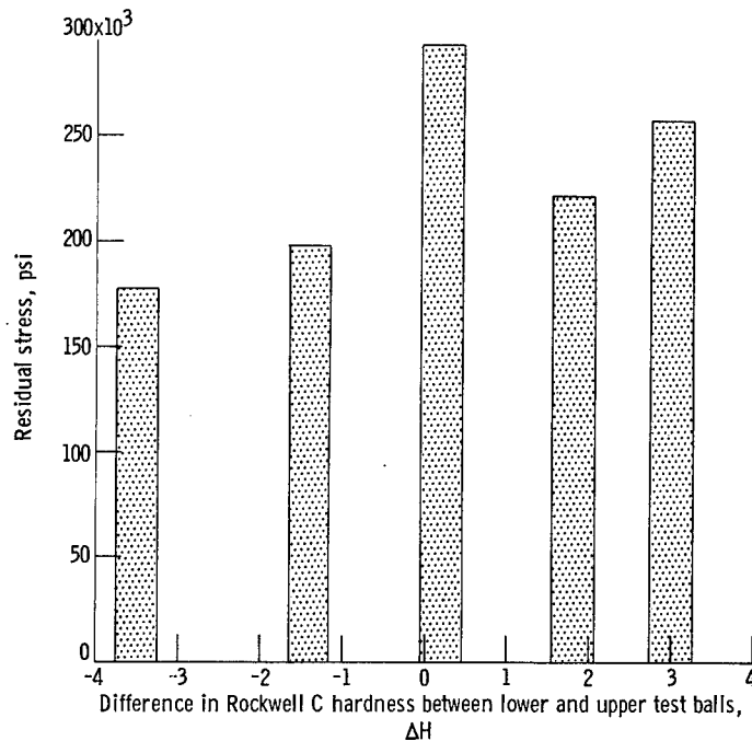
Figure 4. - Measured compressive residual stress in track of upper test balls having Rockwell C hardness of 63.2 as function of \Delta H .
