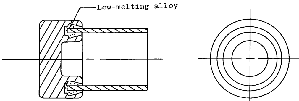
Figure 6.--Chucking method for precision work.
