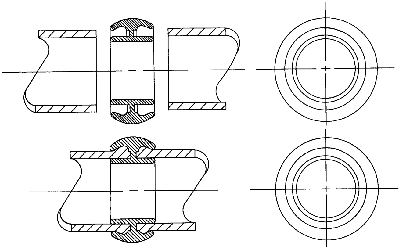
Figure 8.--Pipe connection.
