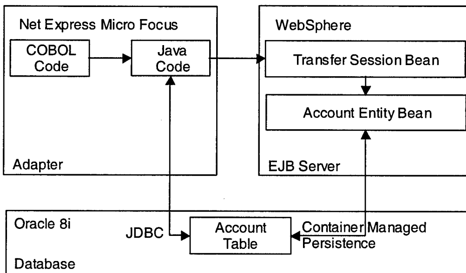
Figure 7: Model Solution Architecture
