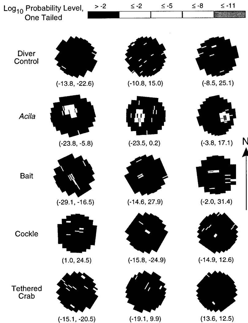
Fig. 4. Plan view of treatment effects at 300 kHz with color-scaled combined probability levels for each treatment replicate. Pixels are 1^\circ in azimuthal and 0.075 m in radial extent. For these treatments, the null hypothesis of no significant change in backscatter intensity was tested one tailed against the anticipated increase. The rough “circle” comprises 221 - 521 pixels (each of 7.5 cm radial and 31-75 cm azimuthal extent) within the 12.5-m 2 search zone. Coordinates are in the two-dimensional Cartesian reference frame shown on the axes of Fig. 2, with origin at the tripod.
