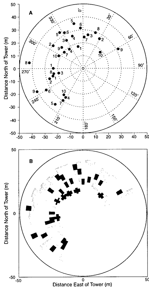
Fig. 2. (A) Scan geometry in both circular and Euclidean coordinates. The open area in the southeast sector of the scan circle was devoted to experiments with buried and proud (unburied), mine-like objects and has been treated elsewhere (Williams, 2001). Filled circles are centered on acoustically-determined (300 kHz) reflector locations, adjacent numbers indicating the treatments applied (1, Acila ; 2, mounds and pits; 3, shrimp; 4, diver control; 5, urchins; 6, bait; 7, cockles; 8, burrows; 9, Molpadia ; 10, tethered crab). (B) Planar plot of the ensounded area at 40 kHz resolution. Pixels are 5^\circ in azimuthal and 0.5 m in radial extent. Black pixels denote treatment locations; grey areas comprise 963 untreated control pixels from which empirical frequency distributions were generated.
