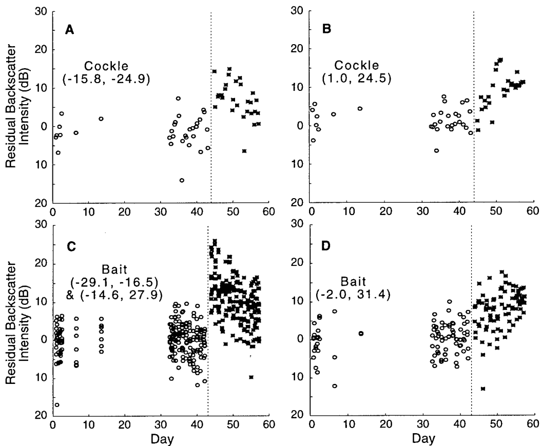
Fig. 6. Time series of 300-kHz backscatter strength for the cockle (top) and bait treatments. Vertical line indicates time of placement of 10 cockles or the bait. (A) Values from a single pixel within the search area of cockle replicate showing an abrupt increase upon placement, followed by linear decay (Kendall's \tau = -0.37 , P = 0.006 , n = 28 ). (B) Values from a single pixel within the search area of cockle replicate in which backscatter strength increased linearly with time (Kendall's \tau = 0.46 , P = 0.001 , n = 28 ). The second centrally located high backscatter pixel within the search area of did not show a statistically significant change over time (Kendall's \tau = -0.15 , P = 0.19 , n = 28 ). (C) Pixels from two replicates combined showing an abrupt increase after placement of the bait, followed by linear decay (Kendall's \tau = -0.28 , P = 0.04 , N = 210 ). (D) The third bait replicate in which backscatter strength increased linearly with time (Kendall's \tau = 0.26 , P = 0.05 , n = 90 ). Probability levels for \tau were deduced from an empirical distribution of 3400 untreated pixels.
