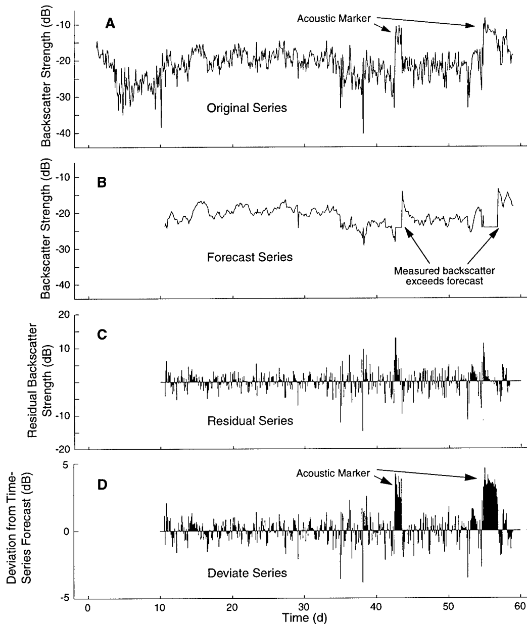
Fig. 9. Original (A), forecast (B), residual (C) and deviate (D) time series showing detection of two markers with sustained backscatter strengths exceeding 4 dB above forecasts. (A) Measured time series. The first 100 scans (10 d) were used to fit an IMA [0,1,1] model. The result: \hat{b}s_{t+1} = 0.25bs_t + 0.75bs_t , SD = 3.5 dB. On detecting a deviation [((\text{original} - \text{forecast})/SD) \geq 2] , the forecast reverts to the series-average backscatter strength of -24.3 dB. (C) The residual series (original - forecast) does not show a coherent pattern, indicating model adequacy, except when outliers are detected. (D) The first marker was retrieved after 10 scans. The second marker remained until the last scan, at which point backscatter strength had diminished slightly. Presence of each marker is clearly distinguishable from background noise.
