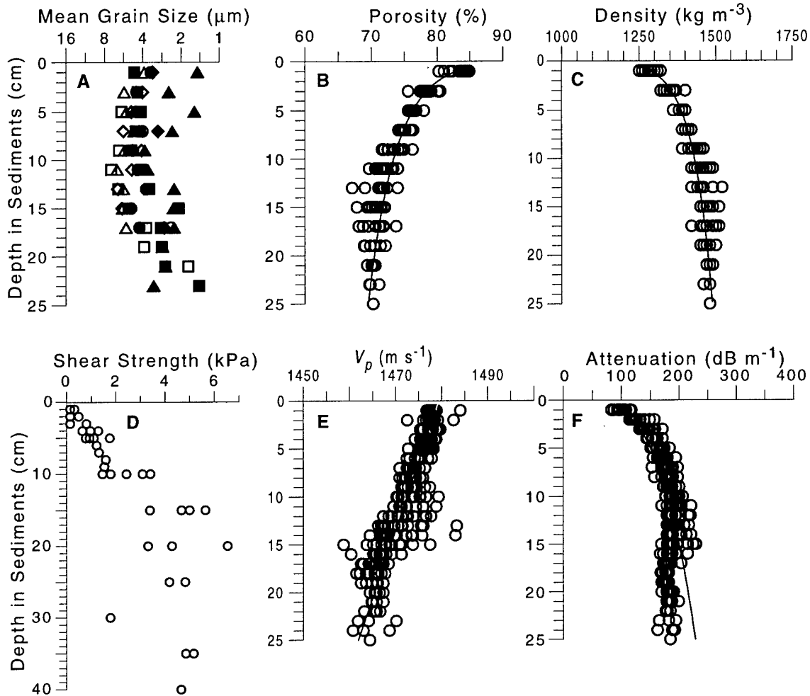
Fig. 10. Geoacoustic properties of West Sound mud. Grain size (A), porosity (B) and bulk density (C) were measured from core samples but shear strength (D) was measured in situ . Sound speed (E) and attenuation (F) versus depth were measured at 400 kHz in diver-collected cores.
