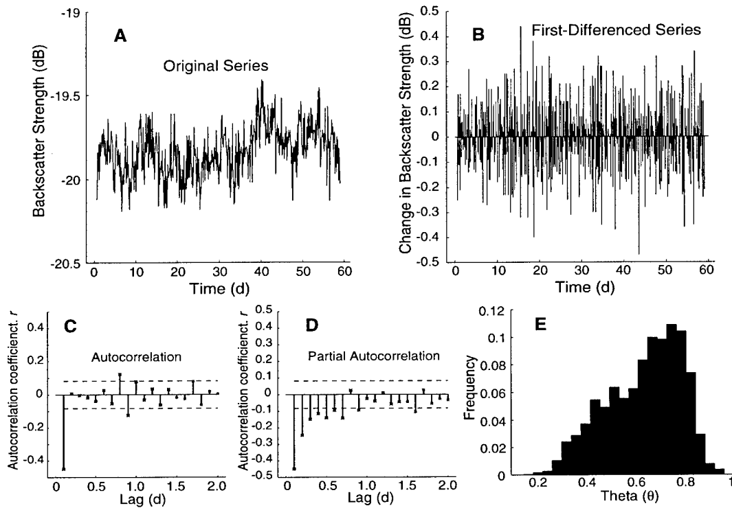
Fig. 8. (A) Time series of 40-kHz average backscatter strength (dB) from the 963 untreated pixels of Fig 2B. (B) First differencing of series A (i.e., change in backscatter strength) removes nonstationarity, giving a stable mean around zero. (C) Autocorrelation and (D) partial autocorrelation functions of the first-differenced series show characteristic behavior of an IMA [0,1,1] model. Dashed lines are \pm 2 standard errors. (E) Frequency distribution of \theta (Eq. 4) fitted to the untreated pixels.
