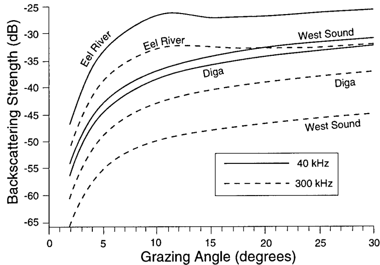
Fig. 12. Backscatter expected from sediments of higher sound-speed contrast, namely those found at Diga, La Spezia, Italy (Richardson, 1997b), and the S60 site at Eel River, California (Richardson, 1997b; Richardson and Briggs, 1993). Predictions use the parameter values of Table 2 and the composite backscatter model of Jackson et al. (1996).
