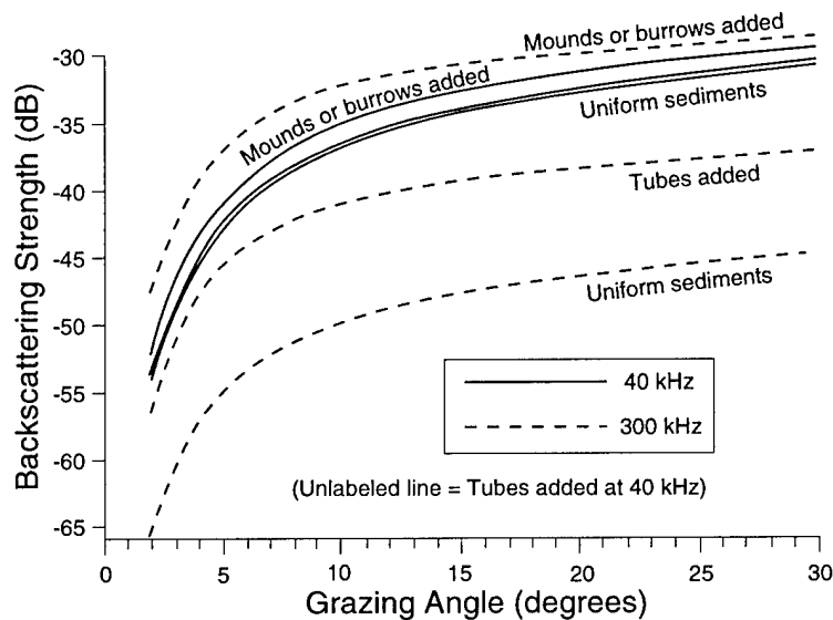
Fig. 11. Backscatter predicted at 40 and 300 kHz from West Sound sediments. Predictions use the parameter values of Table 2 and the composite backscatter model of Jackson et al. (1996).
