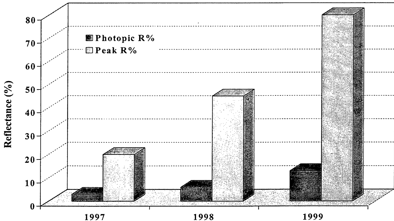
Figure 1. Measured performance improvement in both the peak reflectance and photopic reflectance over the course of the program.
