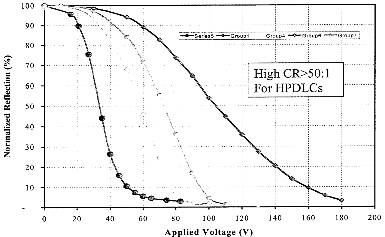
Figure 3. Measured electro-optical performances of HPDLCs with different recipes and curing conditions for 4 \mu\text{m} thick cells.
