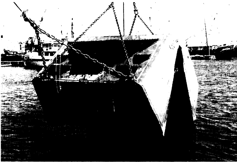
CableArm clamshell
