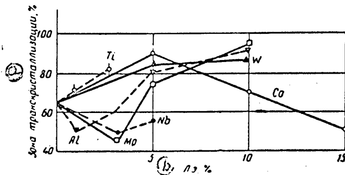
Fig 9. Effect of alloying elements on the width of the transcrystallization zone in the 40 mm section of a stepped specimen of the reference alloy
