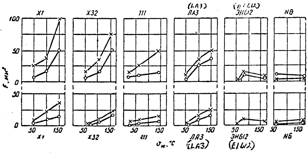
Fig 13. Variation of the grain size of the heat-resistant alloys of practical compositions with superheat \sigma_M and cooling rate in the 40 mm (above) and 20 mm (below) sections; x - hot forms; o - cold forms
