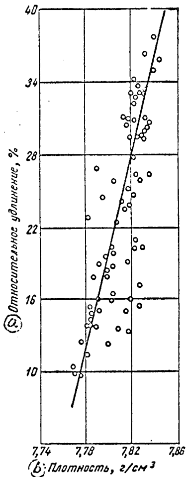
Fig 8. Relation between the density and the plastic properties ( \delta , %) of the XI steel in thin-wall castings a - relative elongation; b - density, g/cm 3
