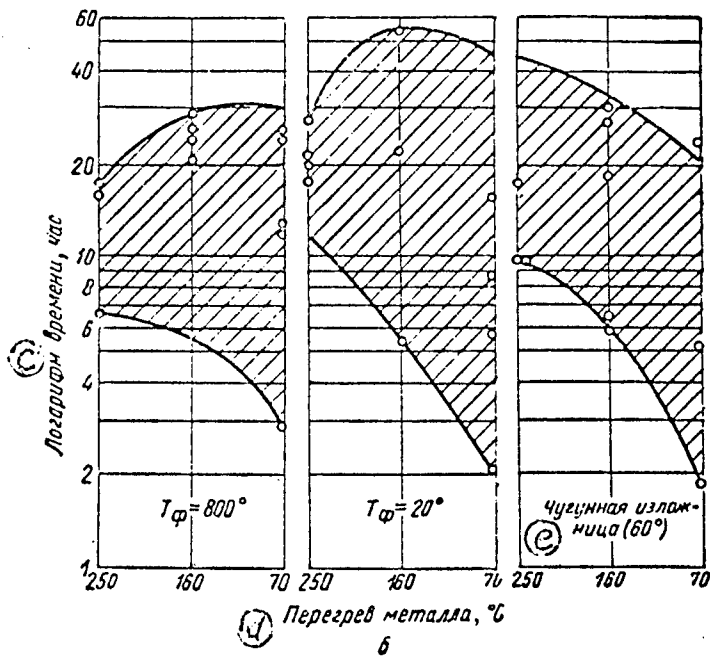
Fig 13. Stress-rupture strength of X1 steel in thin-wall (a) and cloverleaf (b) castings for \sigma_{\tau} = 35 \text{ kg/mm}^2 and T_{\text{test}} = 650^{\circ}\text{C} . c - logarithm of time, hours; d - metal superheat; e - cast iron mold
