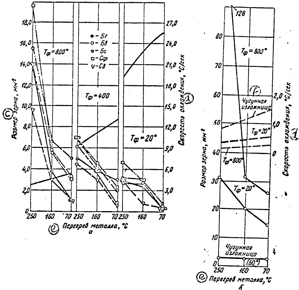
Fig 1. Grain size of the XI steel in the thin-wall (a) and cloverleaf (b) castings
