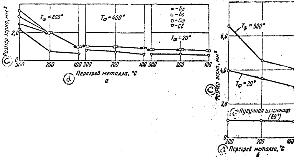
Fig 2. Grain size of the No 6 alloy in thin-wall (a) and cloverleaf (b) castings c - grain size; d - metal superheat; e - cast iron mold
