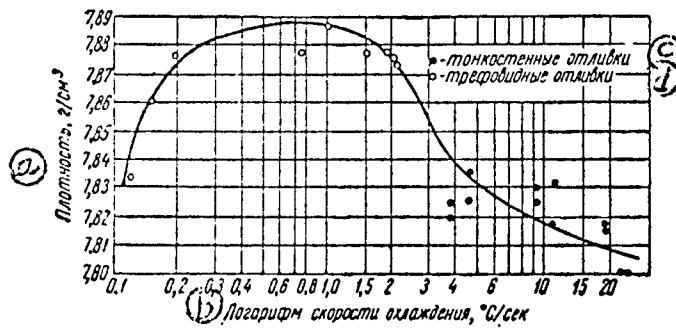
Fig 6. Variation of the steel density as a function of the cooling rate
