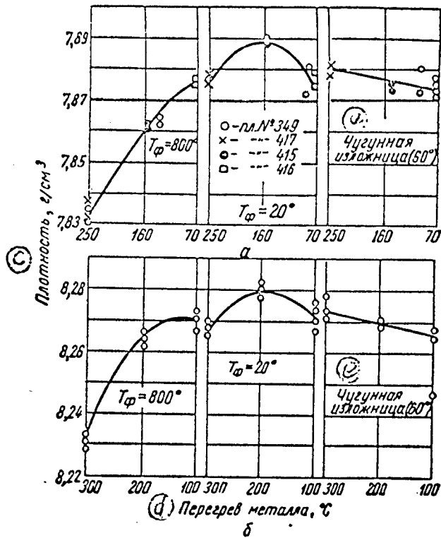
Fig 5. Density of the XI steel (a) and the No 6 alloy (b) in the cloverleaf castings
