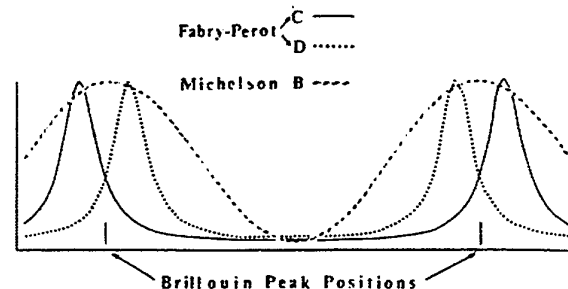
Figure 2.5: This figure represents pass bands for the three interferometers for measuring Brillouin shift. This figure is reported in Hirschberg et al (1984).
