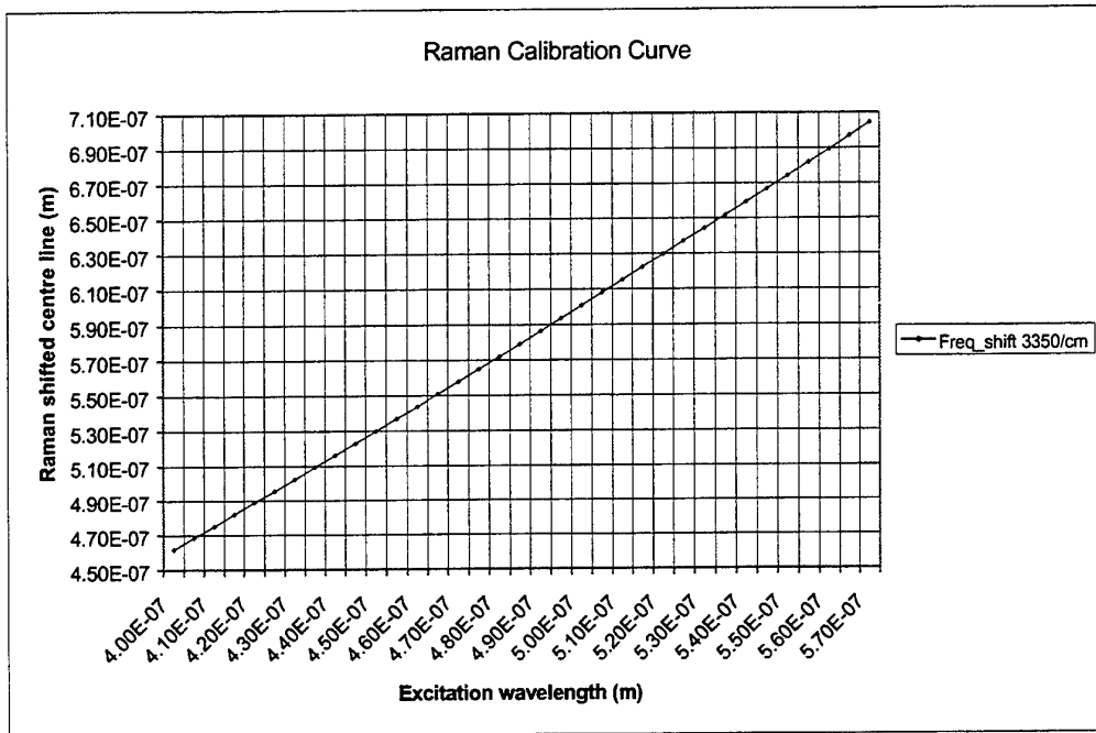
Figure 3.2: Raman calibration curve calculated assuming shift of 3350 wavenumber/cm ( \Delta\nu ). Raman shifted centre line is calculated with the expression \Delta f = c\Delta\nu \cdot 100 . The Raman shifted wavelength has a longer wavelength than the excitation laser.
