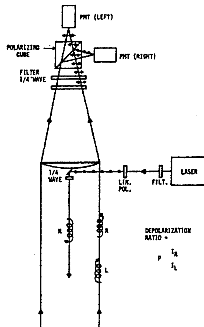
Figure 3.5: Schematic of depth resolved Raman lidar using the circular polarisation method. This is system was proposed by Chang and Young (1975).
