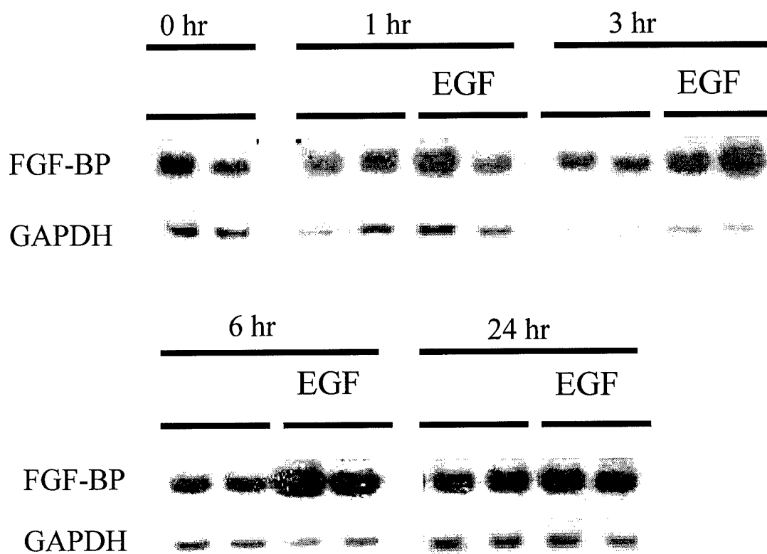
Figure 2. EGF induction of FGF-BP mRNA in MDA-MB-468 cells. Northern blot ( top panel ), quantification of Northern blot ( bottom panel ).
