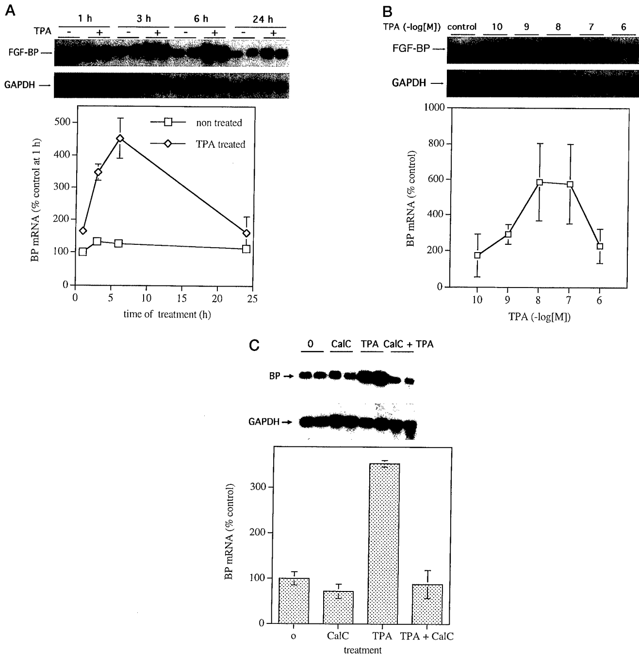
FIG. 1. TPA effect on FGF-BP mRNA in the ME-180 SCC cell line. The respective upper panels for (A–C) are representative Northern blot analyses performed with 30 \mu g of total RNA/lane as described under “Materials and Methods.” Bands corresponding to FGF-BP mRNA (1.2 kb) and the control gene GAPDH mRNA (1.3 kb) are indicated. The respective lower panels (A–C) show results from quantitation of Northern blots. Signal intensities were quantified by phosphorimaging and normalized to the control gene, GAPDH. The mean \pm S.D. of two separate experiments is given. A, time dependence of FGF-BP mRNA induction after exposure to 10^{-7} M TPA. B, concentration dependence of FGF-BP mRNA after 6 h induction by TPA. C, the effect of calphostin C on the TPA induction of FGF-BP mRNA. ME-180 cells were pretreated or not pretreated for 2 h with 10^{-7} M calphostin C (CalC) and then treated for 4 h with or without 10^{-7} M TPA in absence or presence of calphostin C.
