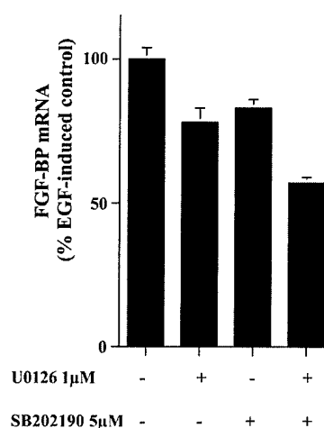
FIG. 7. Additive contribution of ERK and p38 pathways. FGF-BP mRNA levels from ME-180 cells treated with 5 ng/ml EGF for 6 h. Cells were pretreated for 1 h with vehicle alone or with suboptimal concentrations of U0126 (MEK1/2 inhibitor) and/or SB202190 (p38 inhibitor). Northern blot signal intensities of FGF-BP mRNA were quantitated, normalized to GAPDH, and expressed relative to mRNA levels after EGF treatment alone (without inhibitor), which was set to 100%. Basal FGF-BP level (without EGF or inhibitor) was approximately 25%. Values represent the mean and S.D. of at least two separate experiments.
