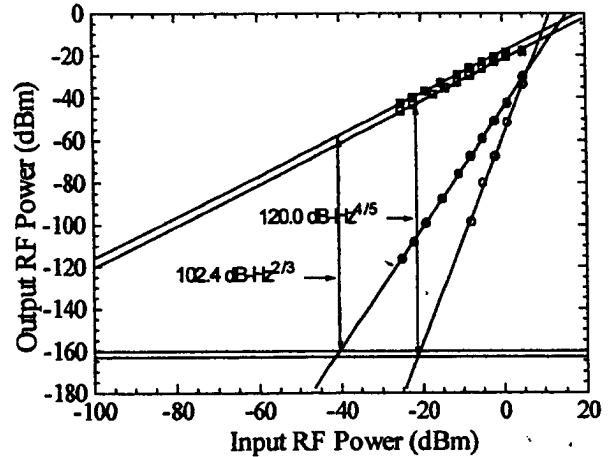
Fig. 3. Two-tone test of the MQW EA photodetector/RF mixer. Converted RF signals ( \blacksquare : for highest slope point, \square : for third-order null point) and the \text{IMD}_3 's ( \bullet : for highest slope point, \circ : third-order null point) are shown.
