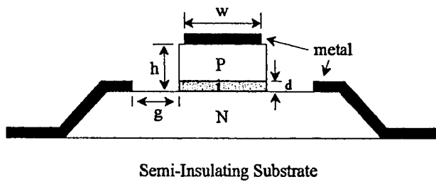
Figure 1. Cross-section of the TW-EAM device. is illustrated in Figure 3. When the terminator impedance Z_L > 50 \Omega , the waveguide inductance will have little impact on the TW-EAM bandwidth; when Z_L = 22 \Omega , in the L_m range of 0.1 nH/mm to 1.0 nH/mm, a larger L_m will yield a larger bandwidth. This suggests that in our device design which uses a low impedance matching approach, a larger inductance L_m would be preferred.
