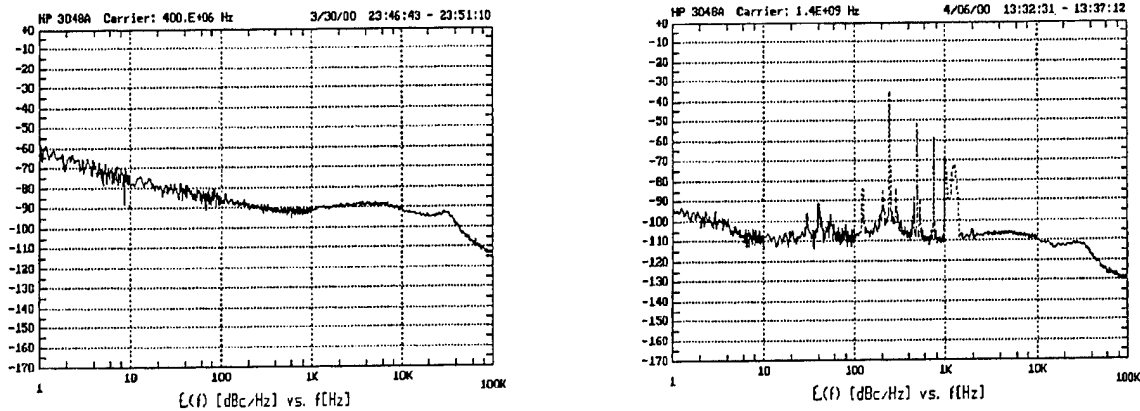
Fig. 7a. Absolute phase noise of the RF source driving the MZM (optical LO generator). b. Residual phase noise characteristic of the EA-OEM up-converted signal at 1.4 GHz
