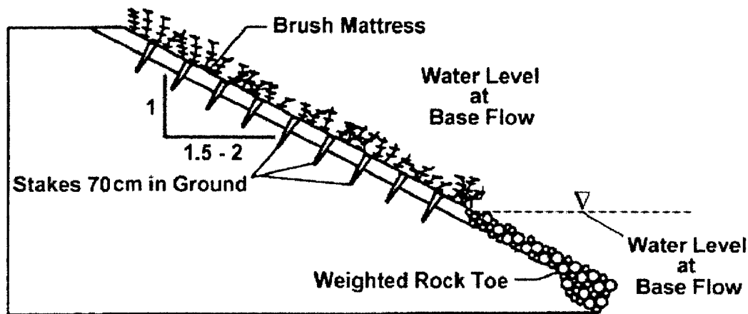
Figure 2. Profile view of brush mattress with rock toe; note relationship to water level at basal flow and that live brush is not permanently flooded
