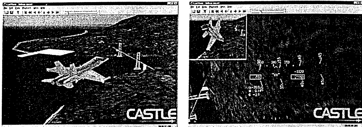
Figure 3. CasView screenshots.
