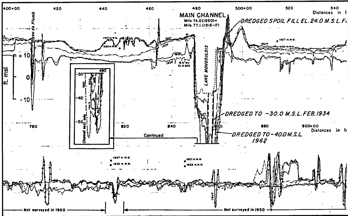
Figure 2-15. Cross-sections taken along transect R-14 showing the amount of sedimentation that has occurred in the vicinity of Bayou Chene in the central portion of the study area. See Figure 2-10 for location (United States Army Corps of Engineers 1974:Plate 223).
