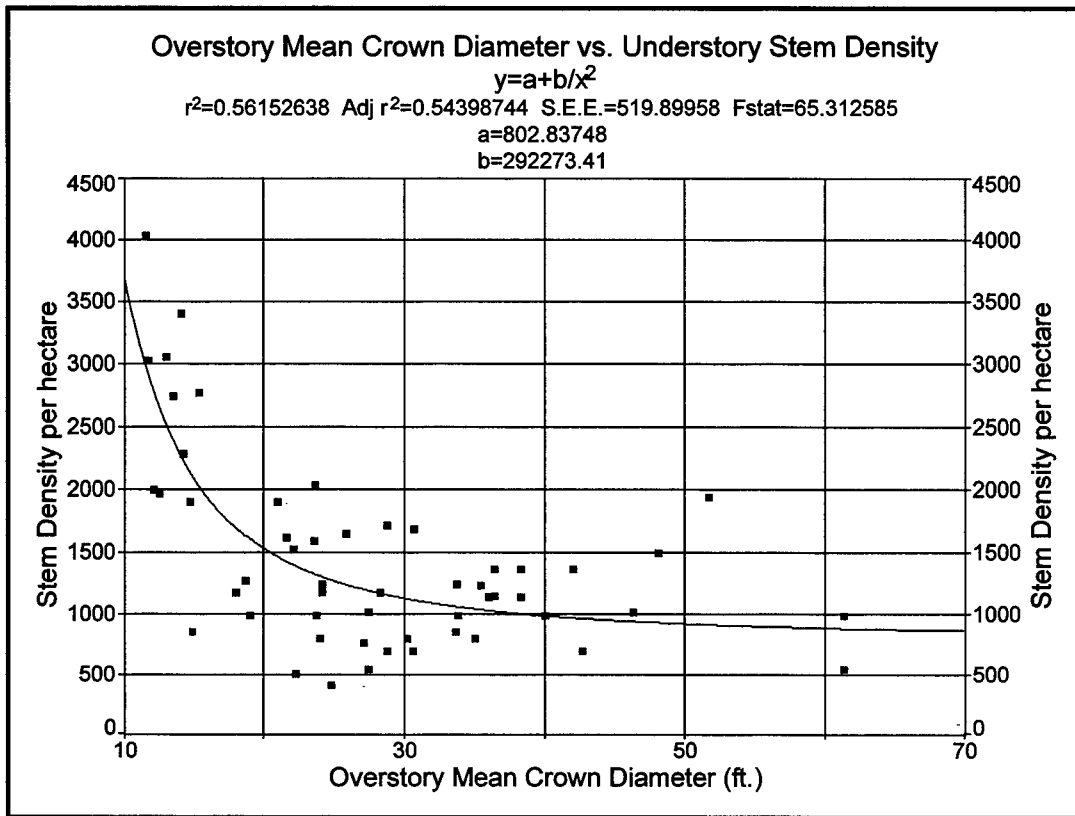
Figure 10. Overstory Mean Crown Diameter vs. Understory Stem Density.
