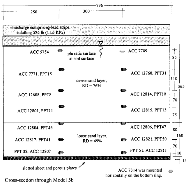
Figure 6. Instrumentation for Model 5b
