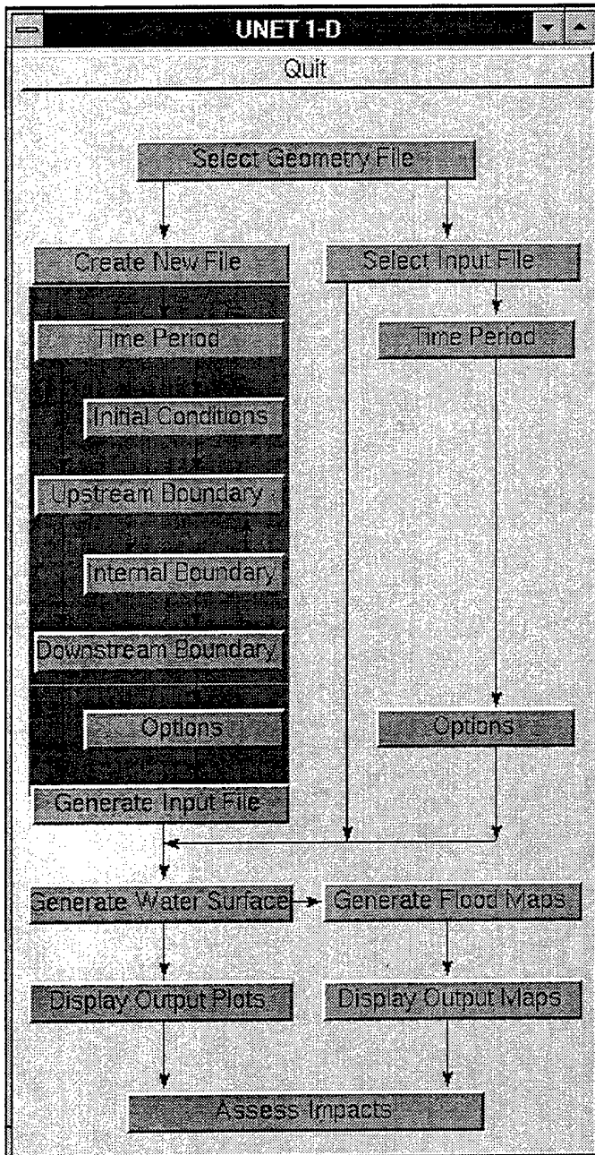
Figure 2. Example Entry Window for UNET
