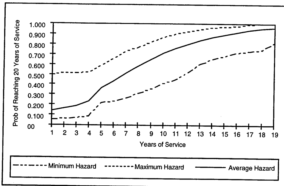
Figure D.1—Dispersion in the Probability of Retirement
