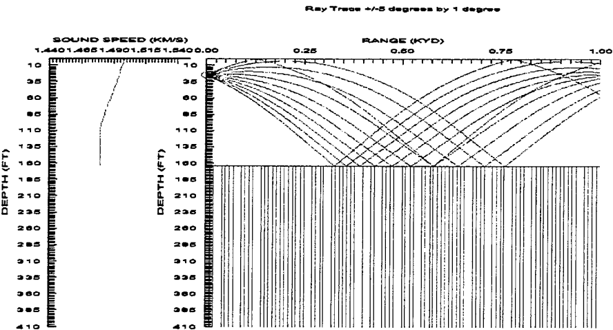
b. Maximum Detection Range (DR) for a 26 ft. Target Depth > 1000 yd, ΔDR >860 yd
