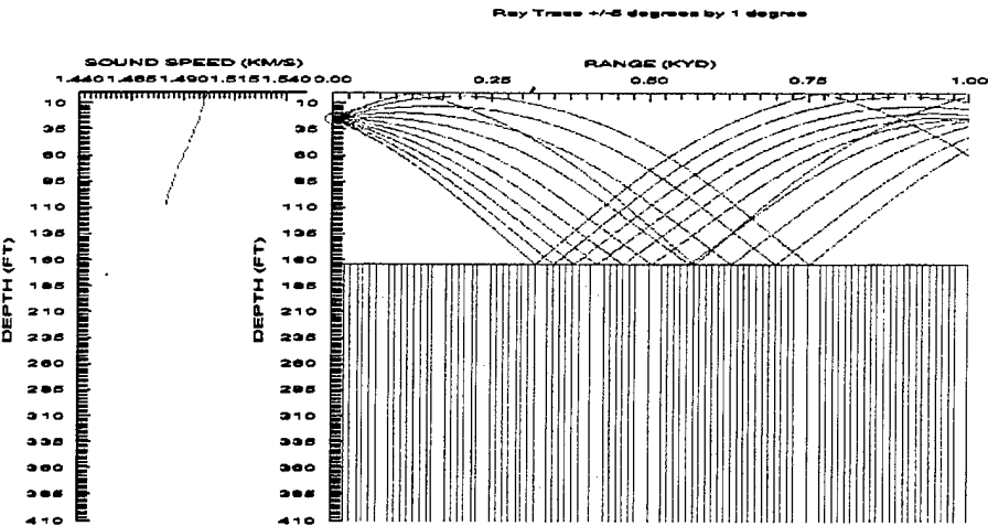
a. Maximum Detection Range (DR) for a 26 ft. Target Depth > 1000 yd, ΔDR >860 yd
