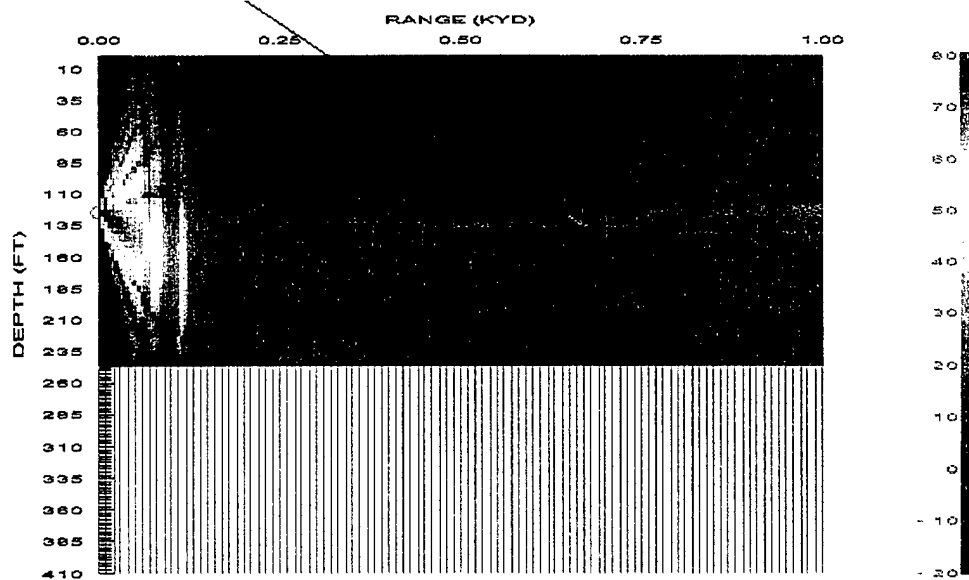
Figure 60. MODAS with -1 m/s Sound Speed error at Source Depth for February 15, 2000, 36.4 N 124.4 E, Mud Bottom, and Source Depth = 125 ft. a. Ray Trace, b. Signal Excess Contour Plot (Max Detection Range at Source Depth >1000 yd, \Delta Max Detection Range at Source Depth >855 yd).
