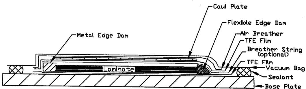
FIGURE C-1. RECOMMENDED LAY-UP TECHNIQUE (WITH FLEXIBLE EDGE DAM)
