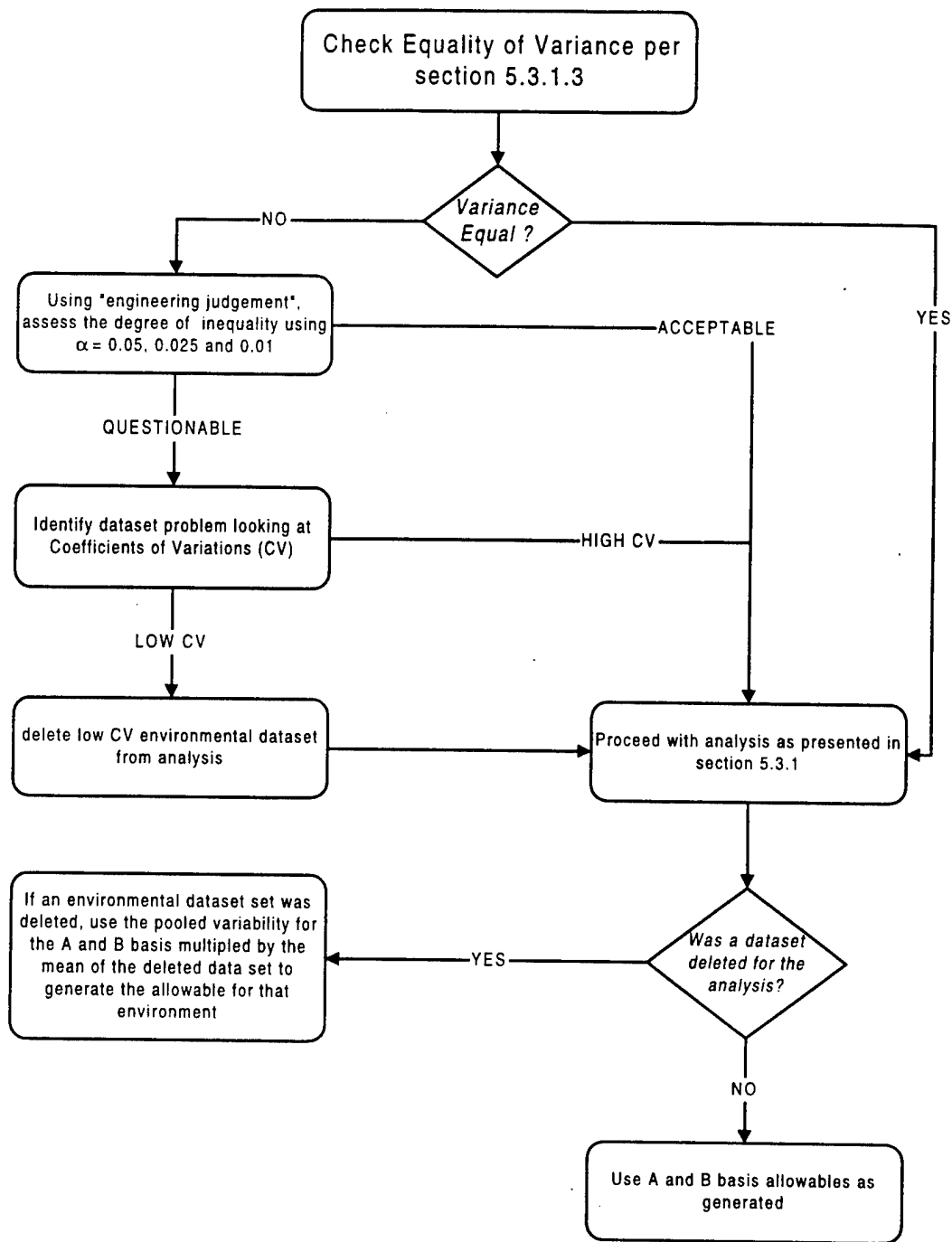
FIGURE 20. PROCEDURES TO OBTAIN DESIGN ALLOWABLES IN THE CASE OF VARIANCE INEQUALITY
