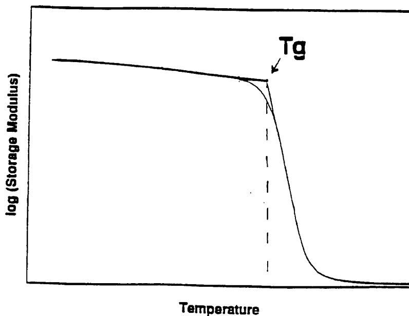
FIGURE 18. GLASS TRANSITION TEMPERATURE DETERMINATION FROM STORAGE MODULUS
