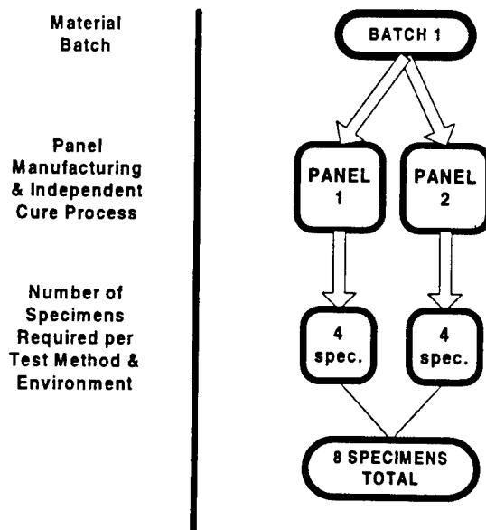
FIGURE 25. AN EXAMPLE OF SPECIMEN SELECTION METHODOLOGY AND PROCESSING TRACEABILITY PER TEST METHOD AND ENVIRONMENTAL CONDITION USED TO ESTABLISH MATERIAL EQUIVALENCE
