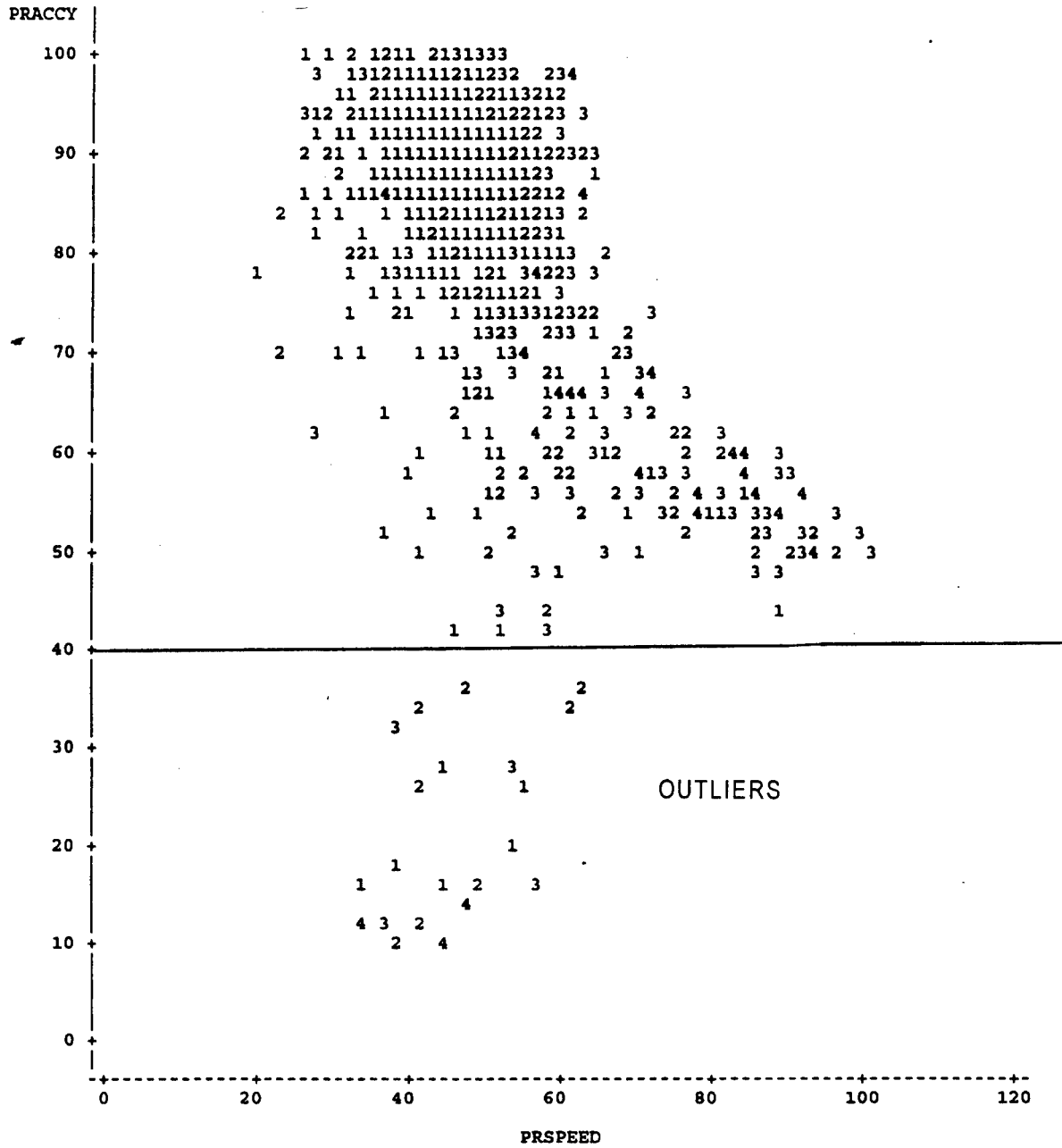
Figure 3.3.1. Plot of PRACCY*PRSPEED. Symbol is value of TRIAL
