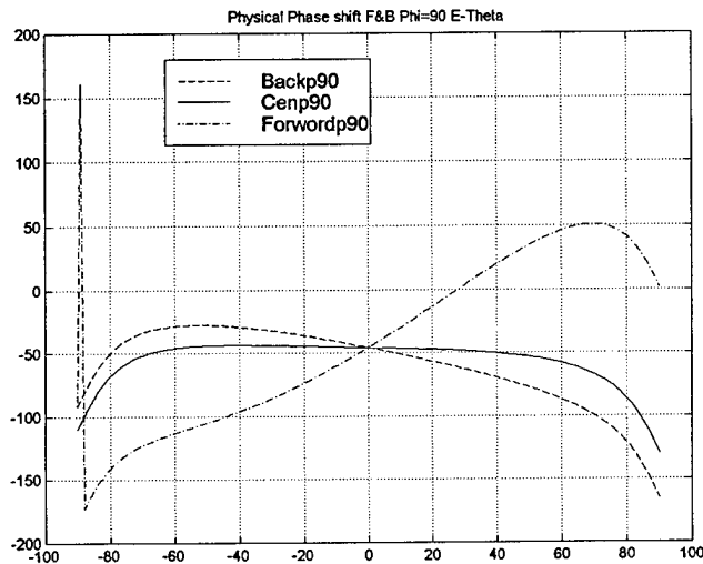
Figure 4 Phased variations in the E- /theta plane.
