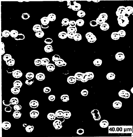
Fig. 8. Deposition in 10 μm filter at a current density of 1 mA/cm 2 pore for 7 hours using configuration in Fig. 2 B.
