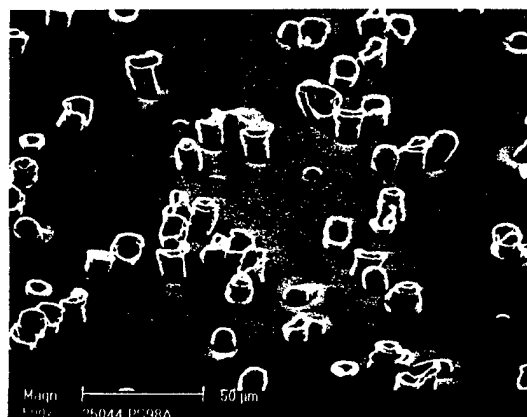
Fig. 18. Remaining structure after dissolution of the 10 \mu\text{m} porous polymeric filter. The Cu "cylinders" were electrochemically deposited by cyclic potentiostatic deposition from a copper pyrophosphate bath at -0.7\text{ V} versus Cu.
