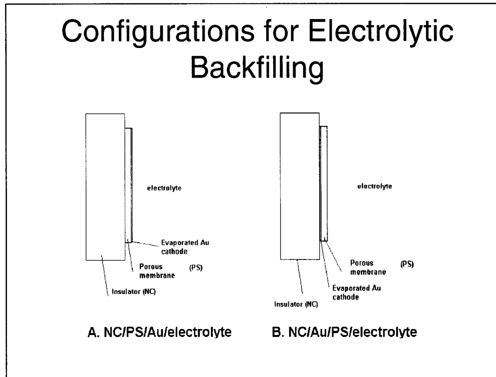
Fig. 2. Configurations for electrolytic backfilling (see text for definition of terms).
