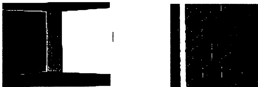
Fig. 20. Micrograph (left photo) of the 2D structure between the electrolyte trough and the gold cathode (mark = 100 mm), and detail (right photo) of the 2D structure (mark = 20 mm).
