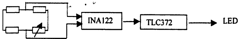
Fig. 9 Scheme of Chemical Sensor Alarm
