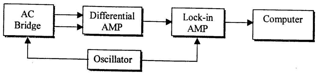
Fig. 8 Scheme of CST-1
