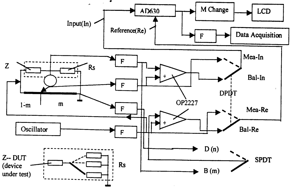
Fig. 7 Scheme of CSIT-1
