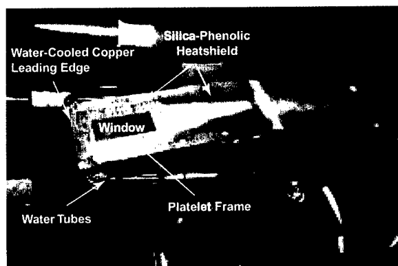
Fig. 2. Slot window-cooling model installation - AEDC HR.
