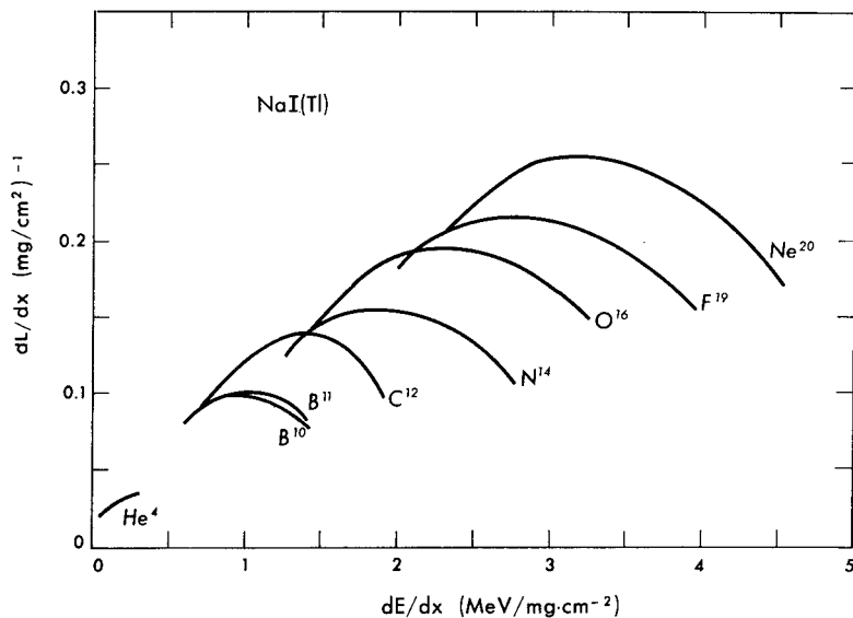
Figure 6. Specific fluorescence of a NaI(Tl) crystal as a function of the total LET. Redrawn from Reference 20. MUB-8234
