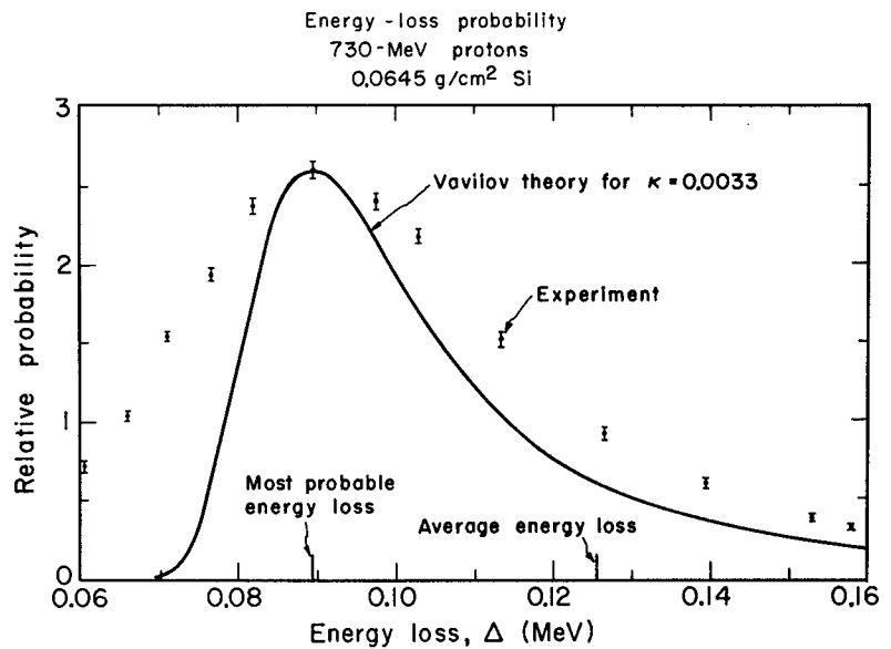
Figure 4. Energy loss probability, 730-MeV protons in 0.0645 g/cm 2 silicon κ = 0.0033. MUB-9085
