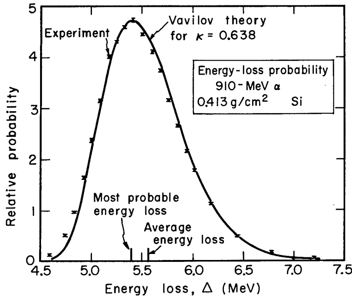
Figure 3. Energy loss probability, 910-MeV alpha particles in 0.413 g/cm 2 silicon κ = 0.638. MUB-9084
