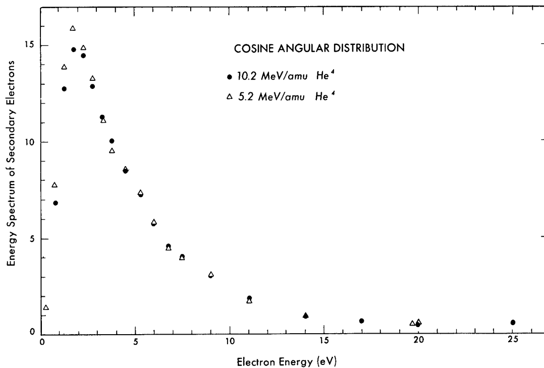
Figure 3. Differential energy spectrum, assuming a cosine angular distribution, for secondary electrons from an Al foil bombarded with 4 He ions. MUB-8231
