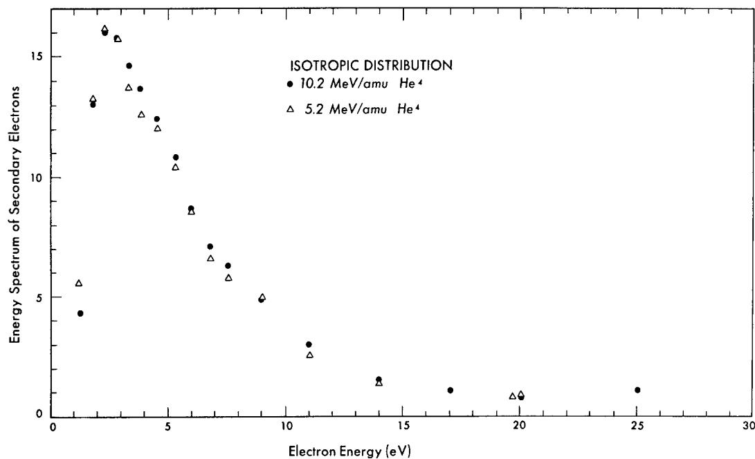
Figure 2. Differential energy spectrum assuming an isotropic angular distribution, for secondary electrons from an Al foil bombarded with 4 He ions. MUB-8230
