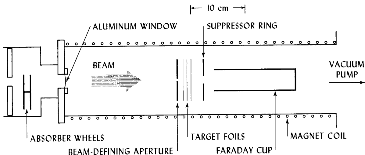
Figure 1. Schematic diagram of the experimental apparatus. MUB-8229
