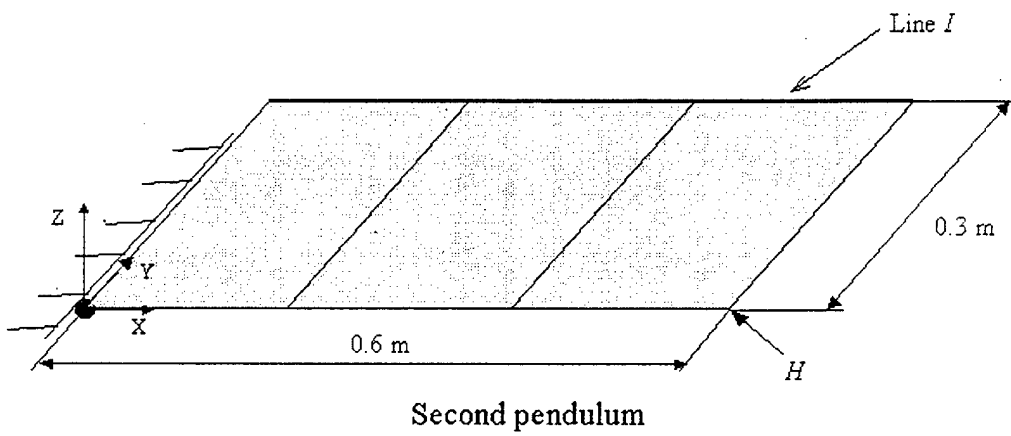
Fig. 6. Pendulum models.
