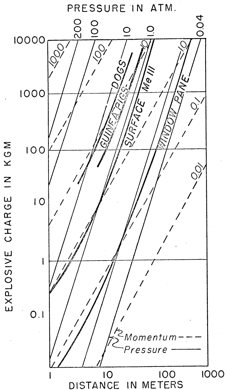
Figure 2 Charge-distance diagram showing characteristic lines of destruction for dogs, guinea pigs, aircraft surfaces, and windowpanes. Solid and broken lines show pressure in atmospheres and momentum in atmosphere-milliseconds, respectively. Modified from Schardin (Reference 42).
