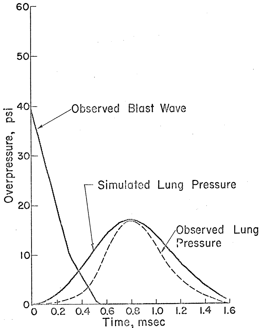
Figure 22 The intrathoracic pressure-time response elicited in a rabbit by a "short"-duration blast wave. Observed data from Clemmedson and Jönsson (Reference 86). Simulated lung-pressure curve after Holladay and Bowen (Reference 82).
