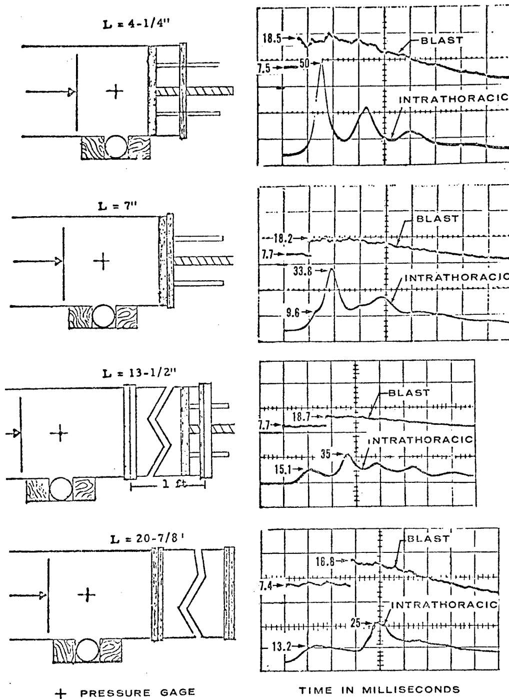
Figure 29 Incident and reflected blast-pressure pulses and intrathoracic pressure-time responses recorded in guinea pigs with an intra-esophageal transducer. Data, courtesy of Mitchell and Gaylord, obtained under the direction of Jones and Richmond (Reference 93); results also used in a recent study by Fletcher (Reference 59).
