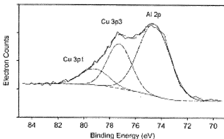
Figure 2. High-resolution ESCA spectrum of a \text{CuAl}_x\text{O}_y film showing the de-convolved peaks for Cu 3p1 at 79.36\text{eV} , Cu 3p3 at 77.43\text{eV} and Al 2p at 74.76\text{eV} .
