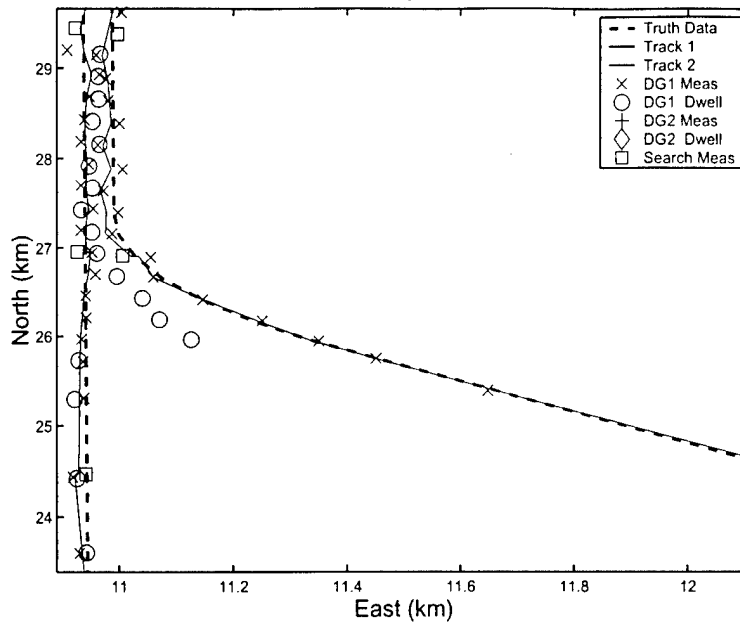
Figure 6. Close up view of tracks after the targets join and the AG/DG technique comes into play.
