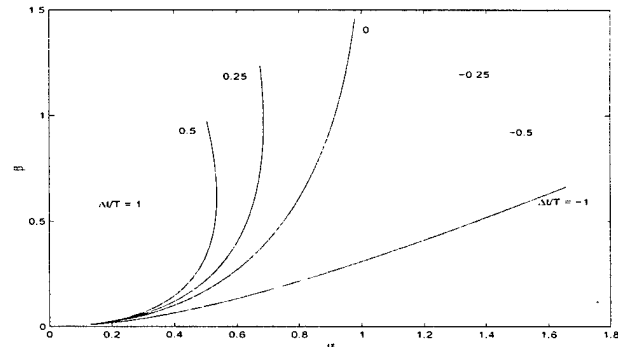
Fig. 6. \beta Versus \alpha with T = 1 s, \sigma_v = 10 m and 0.01 \leq \Gamma \leq 10.0 for various values of \frac{\Delta t}{T}
