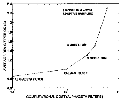
Average Sample Periods versus Computational Cost
