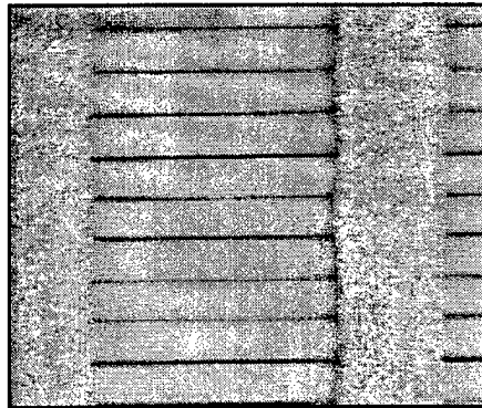
Figure IV-9 (a). PZT-5A Piezoelectric Fibers Used To Make AFC Packs (Courtesy of Continuum Control Corporation)
