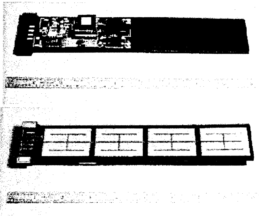
(b) The SmartPack™ Actuator Containing Integrated Electronics
