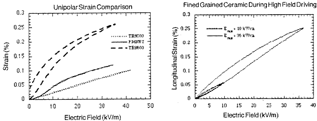
(a) Comparison of Fine-Grained PZT With Conventional PZT and PMN
