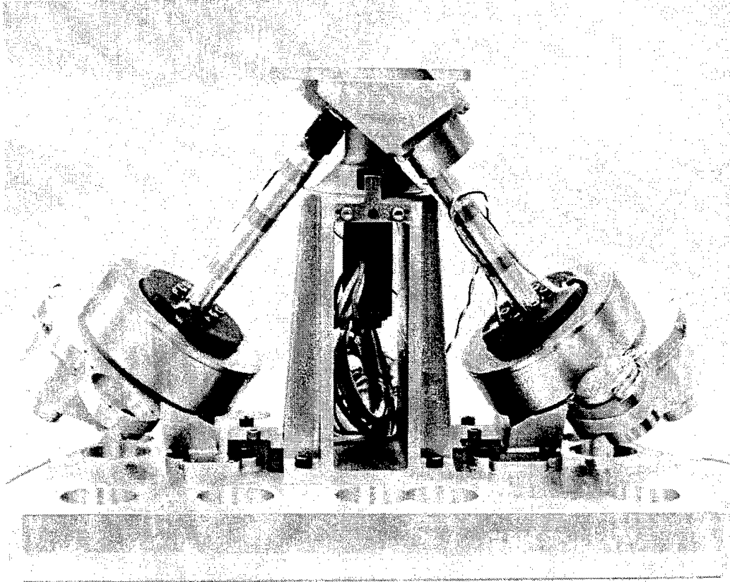
Figure III-5. VISS To Be Launched on the STRV-2 (Courtesy of Honeywell)
