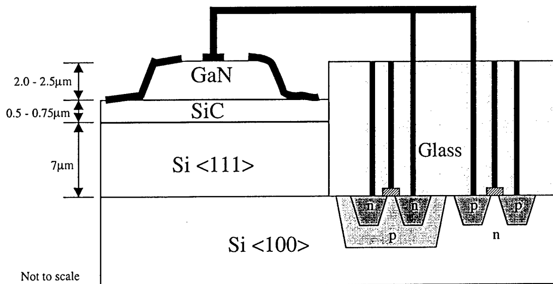
Figure 10. Conceptual Diagram of an Integrated Fabrication Process.
