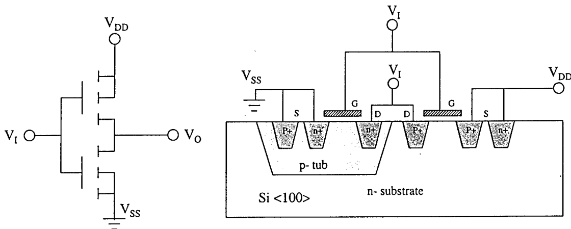
Figure 9. CMOS Inverter.
