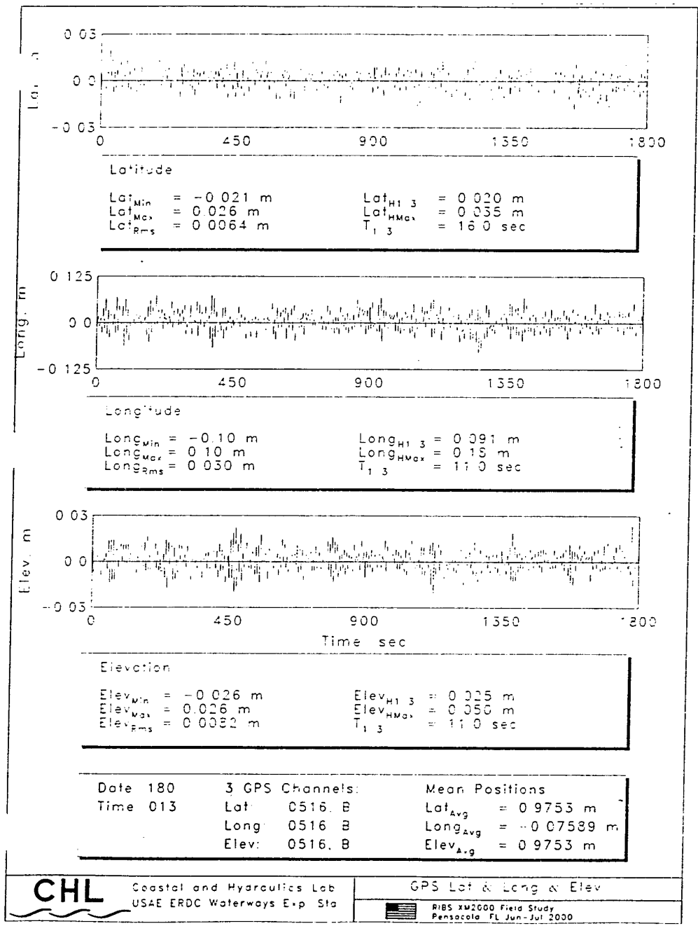
Figure A.7 GEDAP output for GPS (Latitude, Longitude and Elevation) Julian Day 180, hour 013
