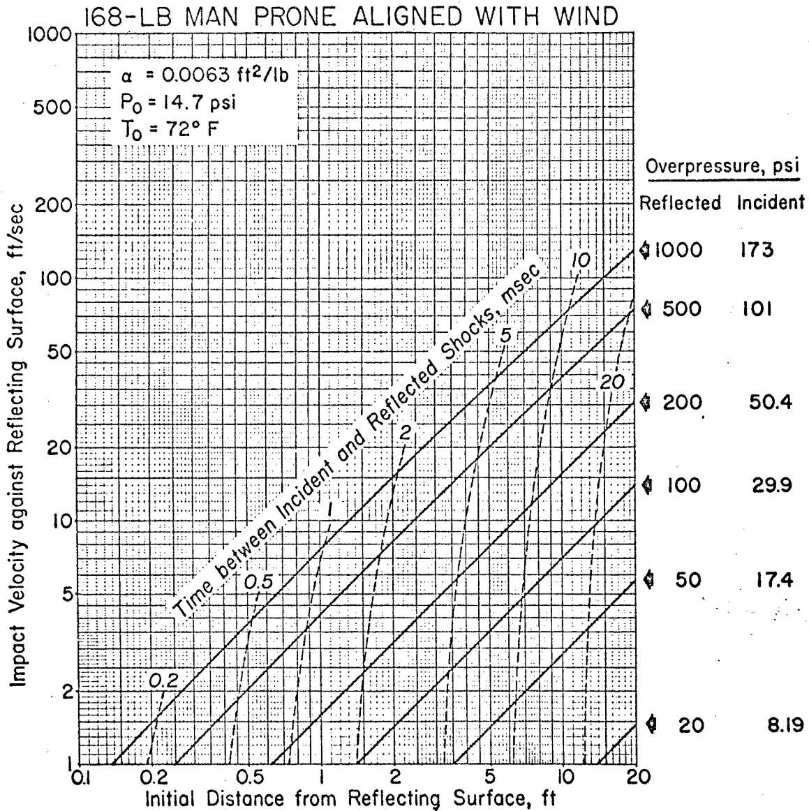
Impact velocity of a man prone aligned ( \alpha = 0.0063 \text{ ft}^2/\text{lb} ) with the winds associated with a square wave, as a function of overpressure and the initial distance of the man from the vertical surface reflecting the blast wave at normal incidence. (Figure from Reference 11.)
