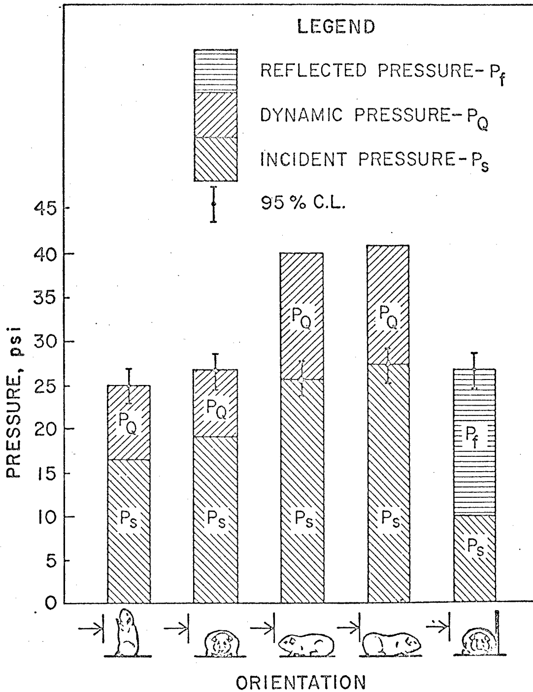
( LD50 Conditions for Guinea Pigs in Various Orientations. Measurements Were Made at Ambient Pressure of 12 Psia. Figure from Reference 21.)
