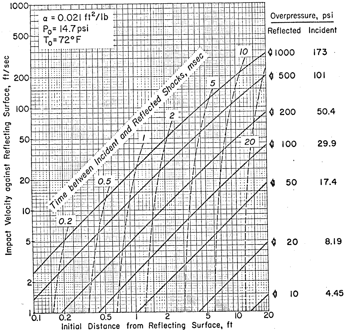
Impact velocity of a man crouching broadside, standing sidewise, or prone perpendicular ( a = 0.021 \text{ ft}^2/\text{lb} ) to the winds associated with a square wave, as a function of overpressure and the initial distance of the man from the vertical surface reflecting the blast wave at normal incidence. (Figure from Reference 11.)
