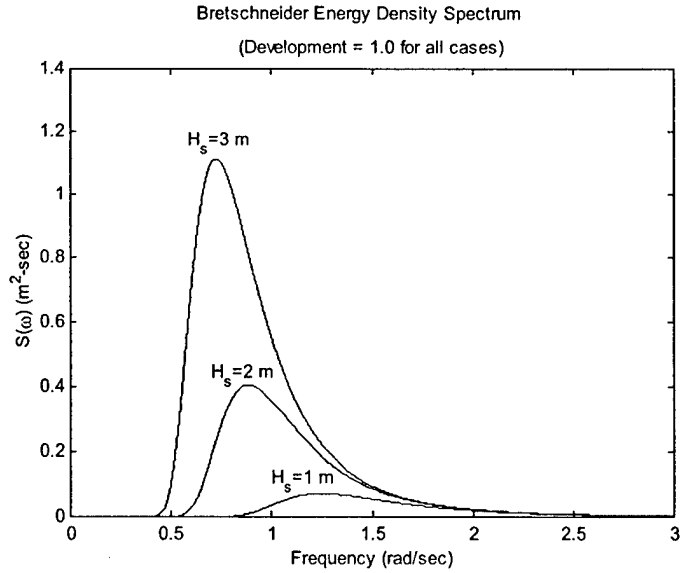
Figure 2-3: Bretschneider Spectrum for Varying Sea Severity
