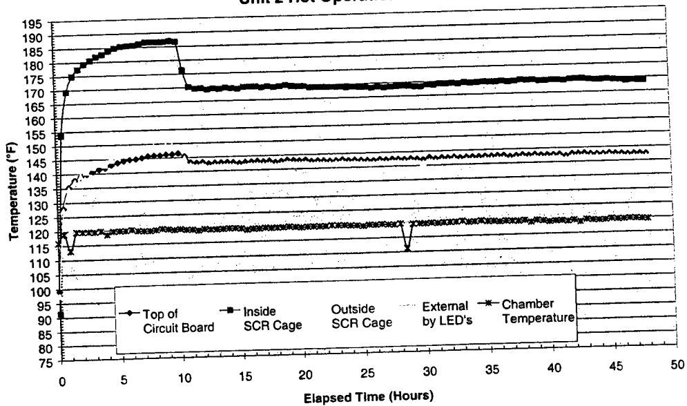
FIGURE 8: Series 2 Temperature profiles for Hot Operation Testing (a) Unit 1 (b) Unit 2
