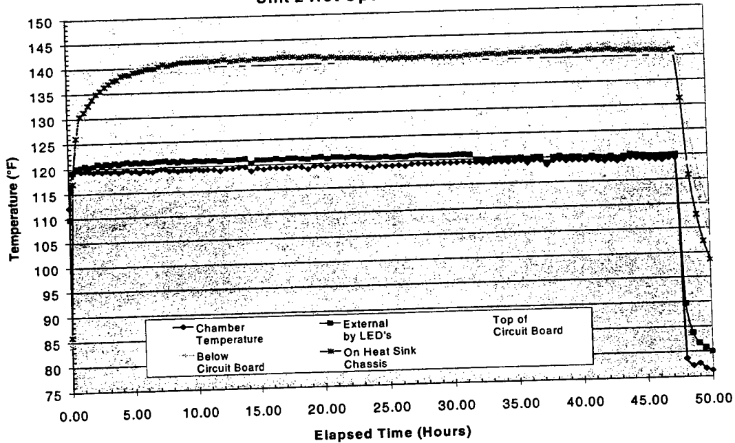
FIGURE 1: Temperature Profiles During Hot Operation Testing of the GFI Units (a) Unit 1 (b) Unit 2
