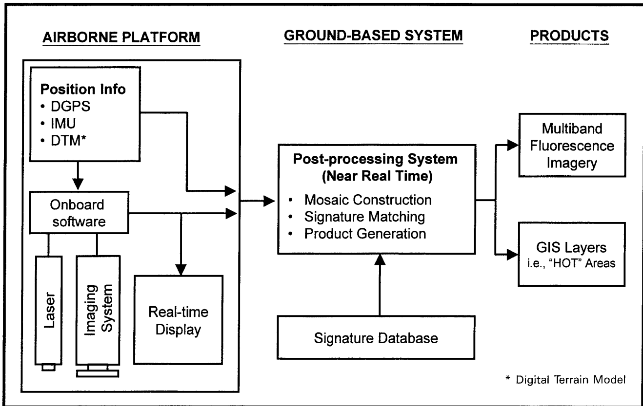
Figure 2. Block diagram of airborne and ground-based components
