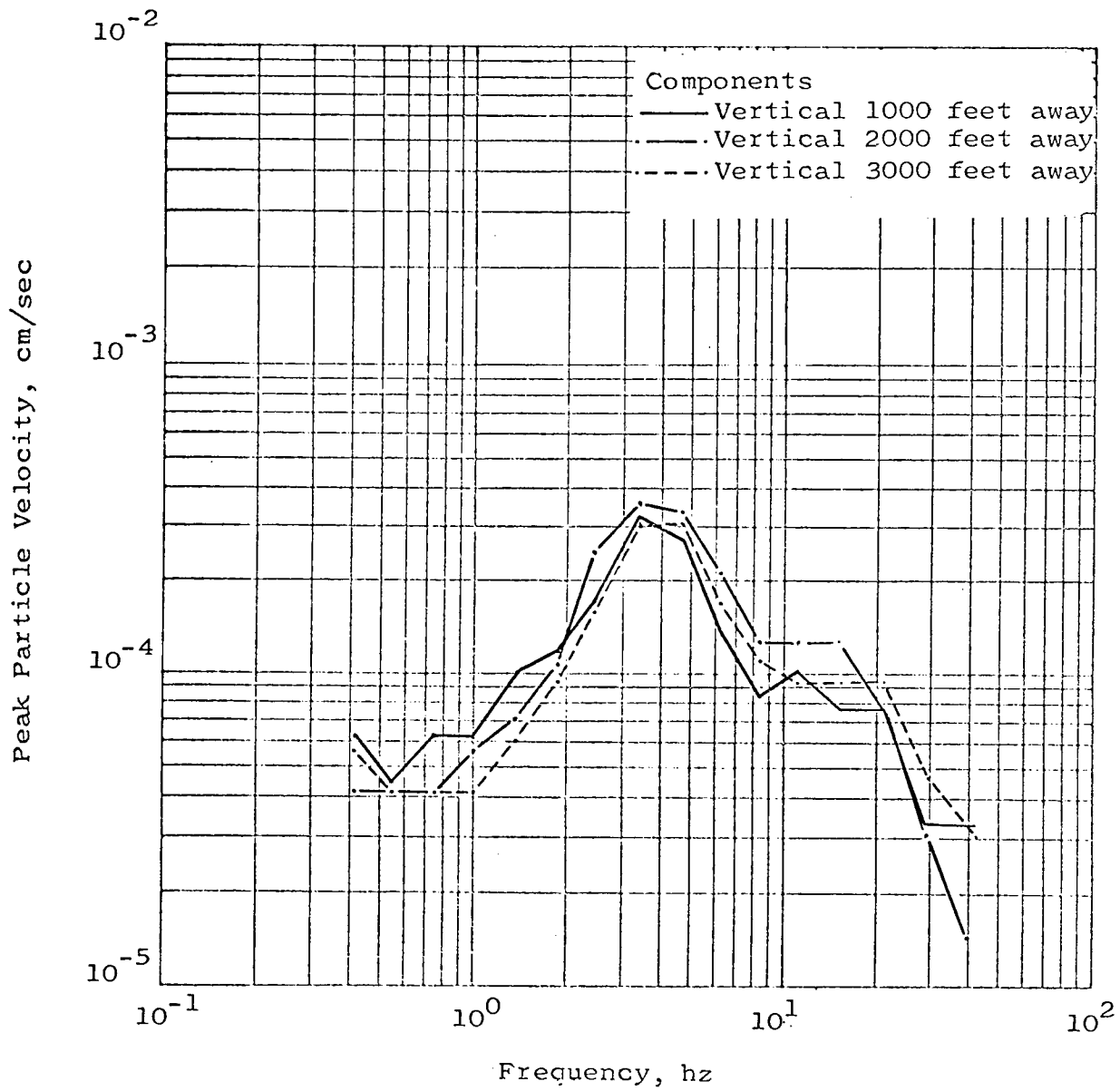
Figure 3.16 Peak Band-Pass Filtered Particle Velocity versus Frequency, Station 20S
