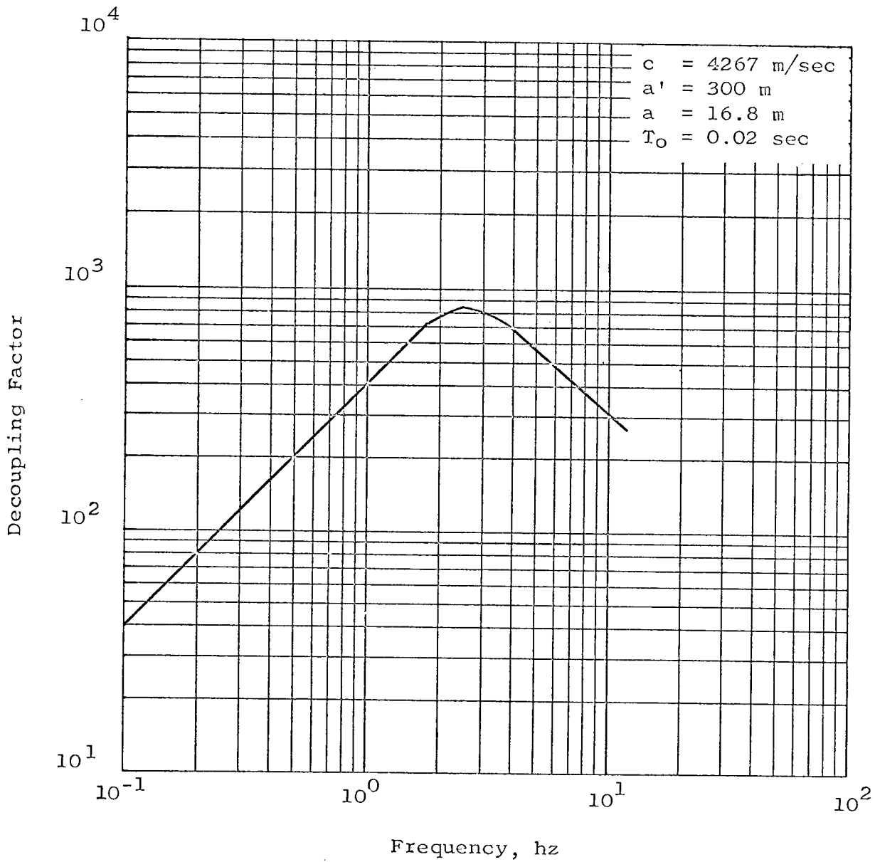
Figure 4.13 Decoupling Factor for Interpolation Function Pressure Profile, p(t) = p \text{ sinc } \tau H(\tau)
