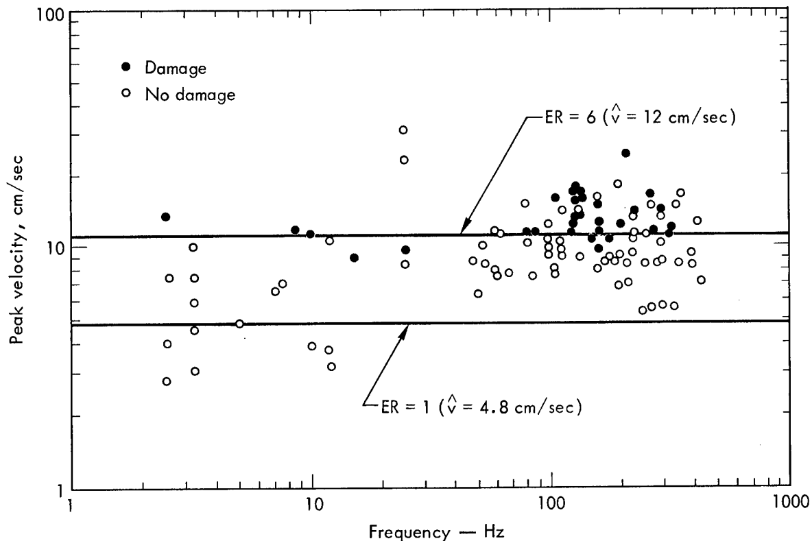
Fig. 1. First estimates of damage threshold, based on peak surface velocity. ER (energy ratio) defined as A^2/F^2 , where A = acceleration in \text{ft}/\text{sec}^2 and F = frequency in Hz.
